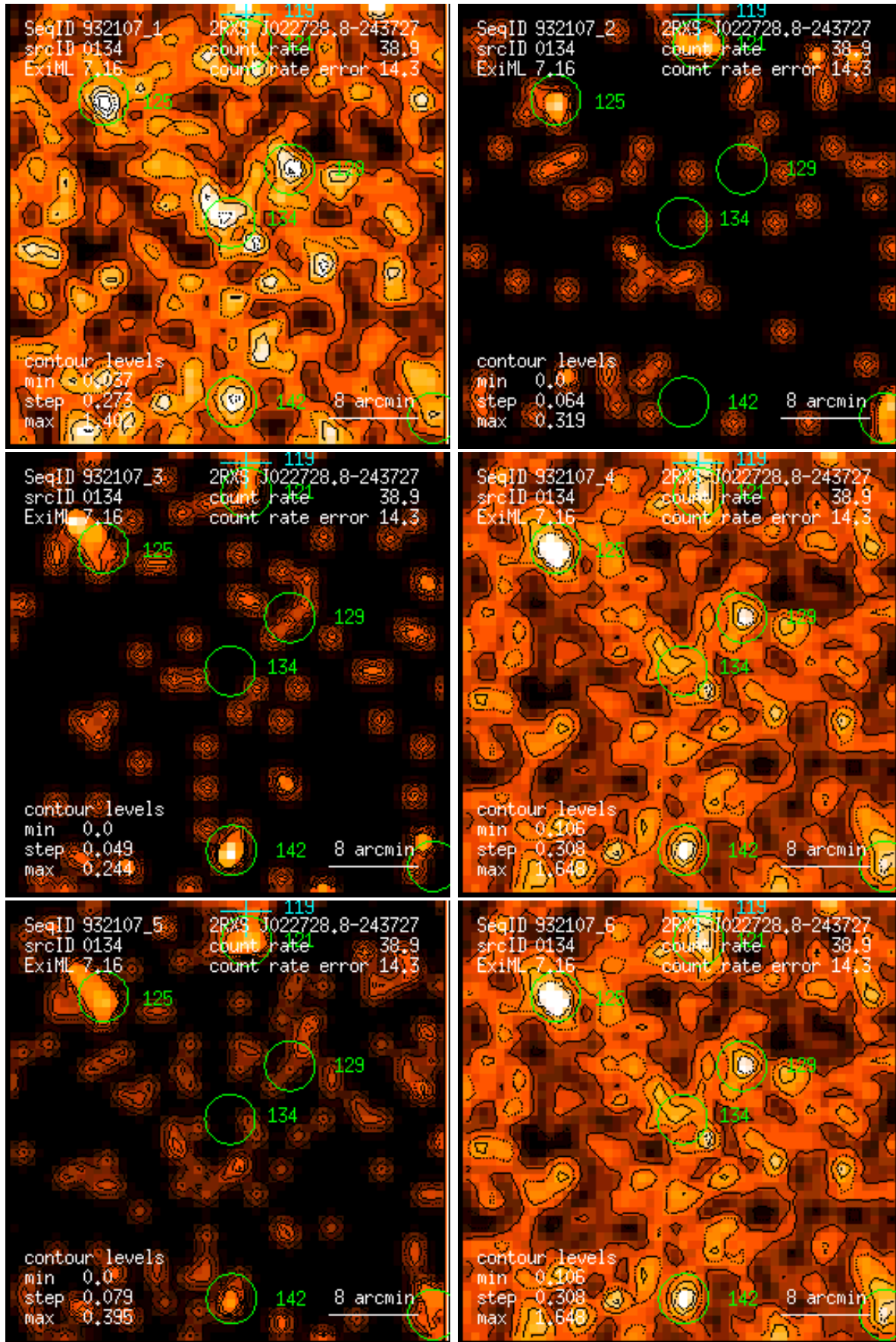
Figure 134: RASS 932107: detection 0134: band rate images, Gaussian filter: (1) PSPC channels 11 – 41, (2) 52 – 90, (3) 91 – 201, (4) 11 – 235, (5) 52 – 201, (6) 11 – 201. Broad band rates in counts/ks. Band rate contour levels in counts/ks/arcmin 2 .
