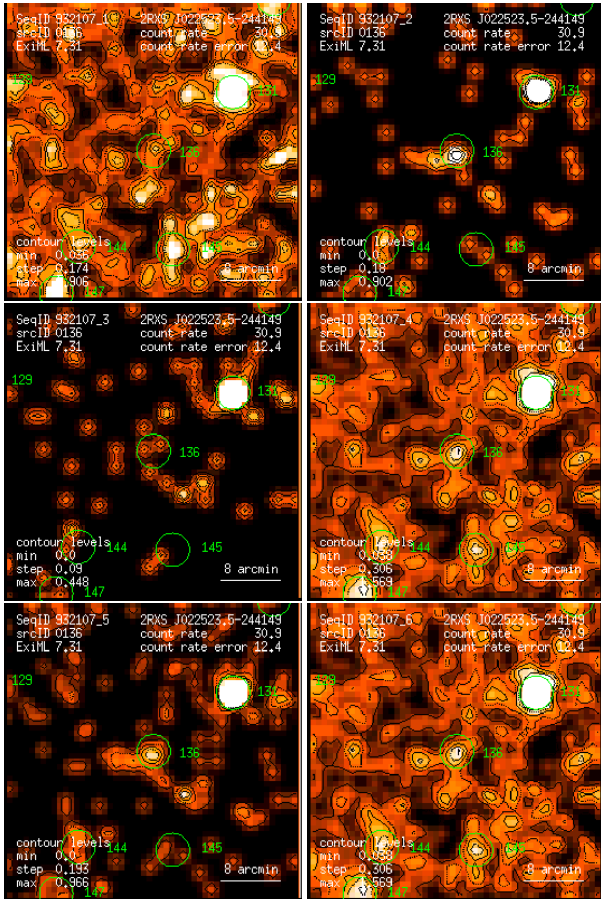
Figure 136: RASS 932107: detection 0136: band rate images, Gaussian filter: (1) PSPC channels 11 – 41, (2) 52 – 90, (3) 91 – 201, (4) 11 – 235, (5) 52 – 201, (6) 11 – 201. Broad band rates in counts/ks. Band rate contour levels in counts/ks/arcmin 2 .
