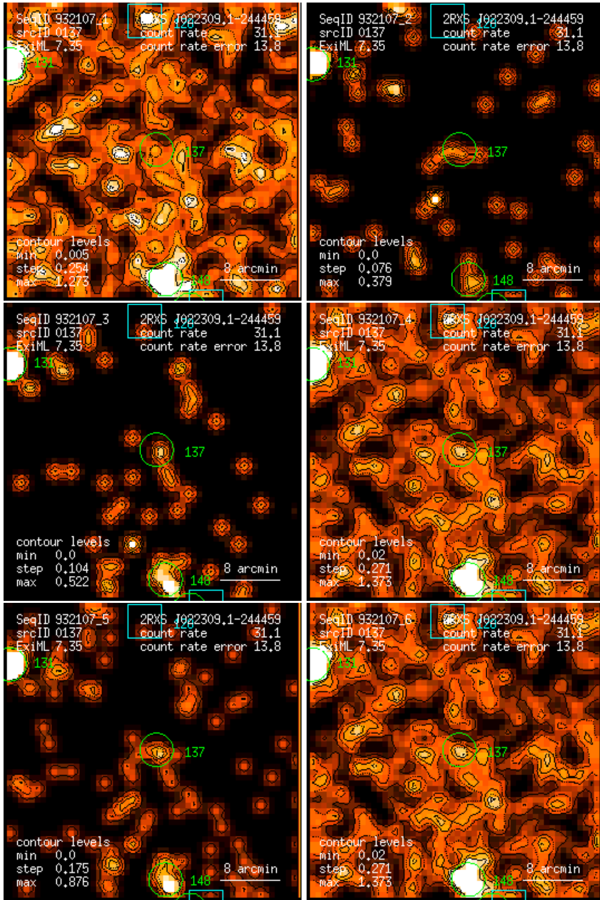
Figure 137: RASS 932107: detection 0137: band rate images, Gaussian filter: (1) PSPC channels 11 – 41, (2) 52 – 90, (3) 91 – 201, (4) 11 – 235, (5) 52 – 201, (6) 11 – 201. Broad band rates in counts/ks. Band rate contour levels in counts/ks/arcmin 2 .
