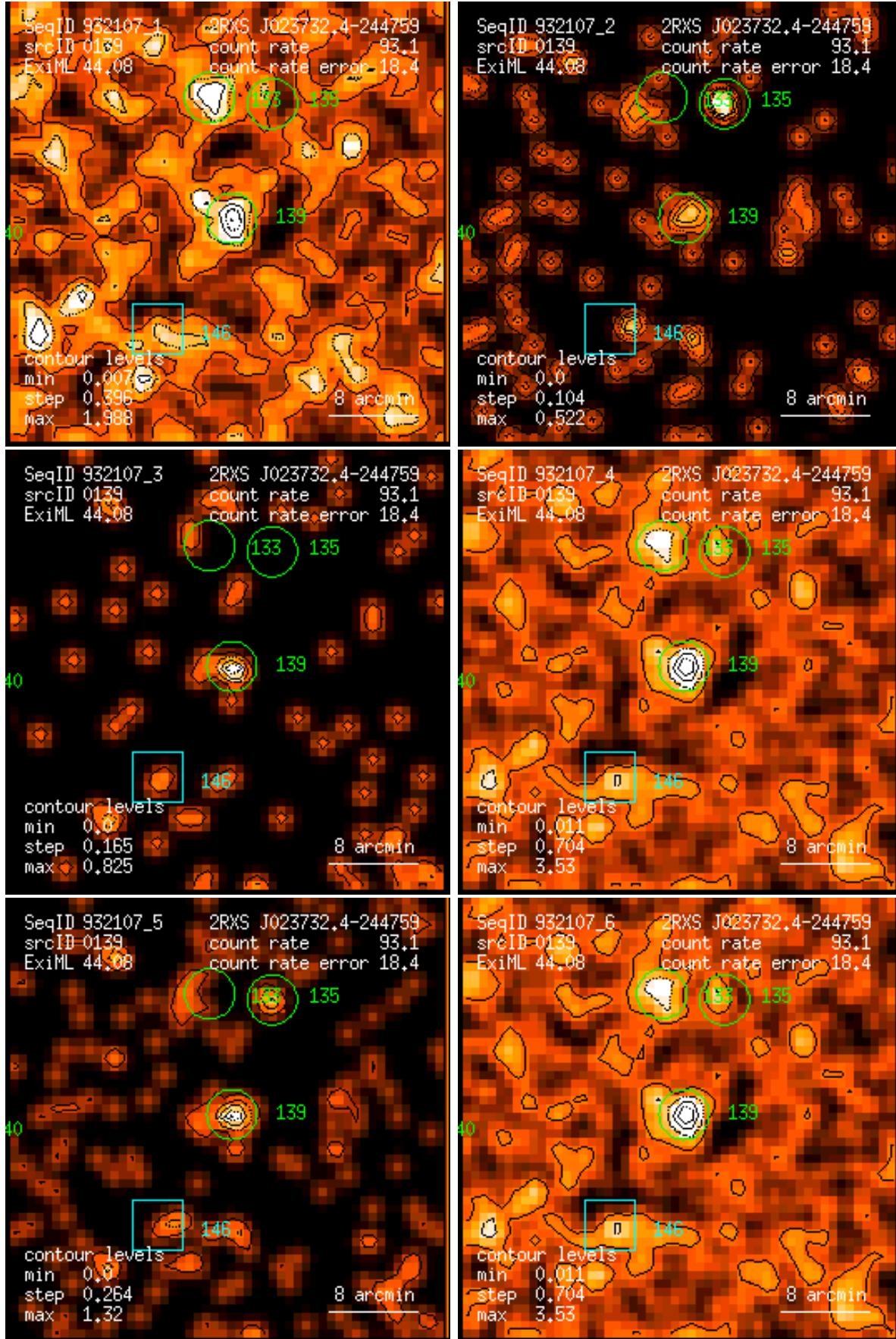
Figure 139: RASS 932107: detection 0139: band rate images, Gaussian filter: (1) PSPC channels 11 – 41, (2) 52 – 90, (3) 91 – 201, (4) 11 – 235, (5) 52 – 201, (6) 11 – 201. Broad band rates in counts/ks. Band rate contour levels in counts/ks/arcmin 2 .
