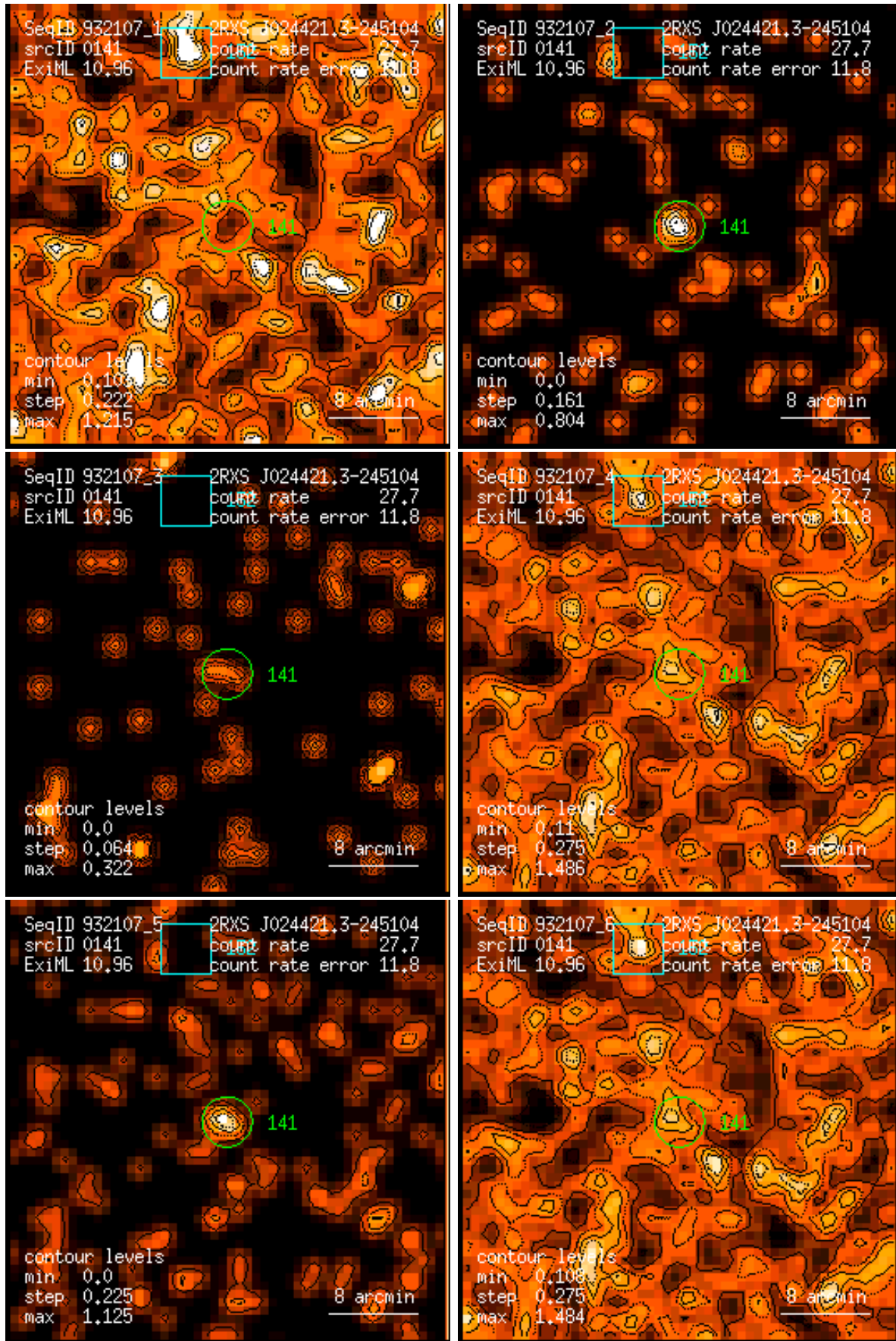
Figure 141: RASS 932107: detection 0141: band rate images, Gaussian filter: (1) PSPC channels 11 – 41, (2) 52 – 90, (3) 91 – 201, (4) 11 – 235, (5) 52 – 201, (6) 11 – 201. Broad band rates in counts/ks. Band rate contour levels in counts/ks/arcmin 2 .
