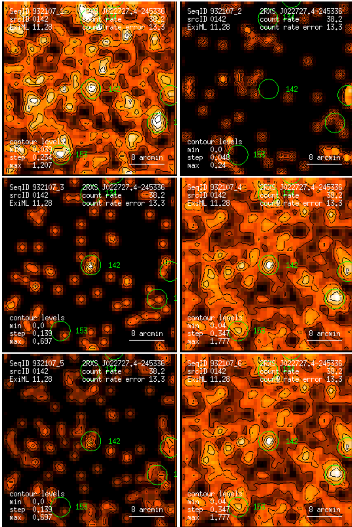
Figure 142: RASS 932107: detection 0142: band rate images, Gaussian filter: (1) PSPC channels 11 – 41, (2) 52 – 90, (3) 91 – 201, (4) 11 – 235, (5) 52 – 201, (6) 11 – 201. Broad band rates in counts/ks. Band rate contour levels in counts/ks/arcmin 2 .
