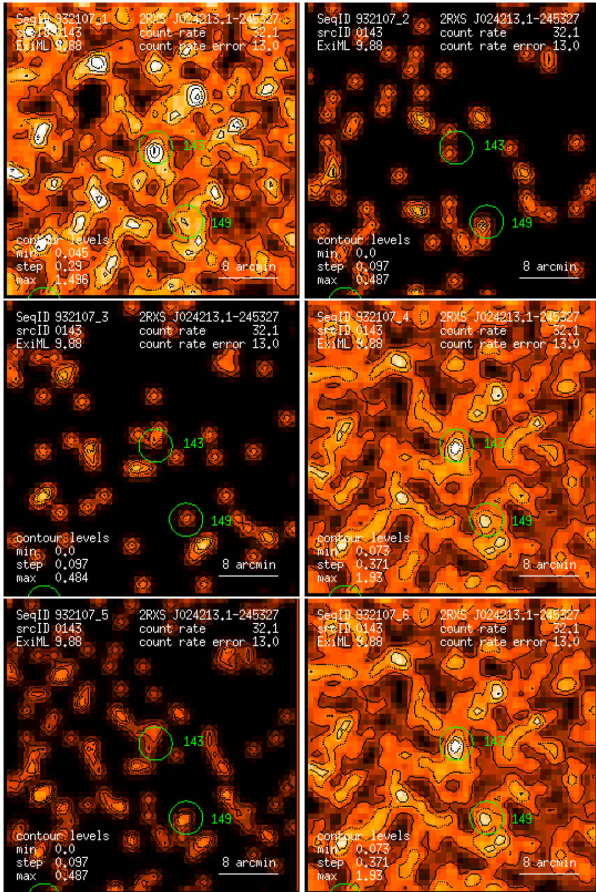
Figure 143: RASS 932107: detection 0143: band rate images, Gaussian filter: (1) PSPC channels 11 – 41, (2) 52 – 90, (3) 91 – 201, (4) 11 – 235, (5) 52 – 201, (6) 11 – 201. Broad band rates in counts/ks. Band rate contour levels in counts/ks/arcmin 2 .
