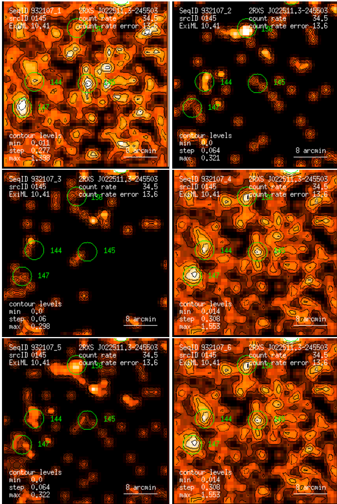
Figure 145: RASS 932107: detection 0145: band rate images, Gaussian filter: (1) PSPC channels 11 – 41, (2) 52 – 90, (3) 91 – 201, (4) 11 – 235, (5) 52 – 201, (6) 11 – 201. Broad band rates in counts/ks. Band rate contour levels in counts/ks/arcmin 2 .
