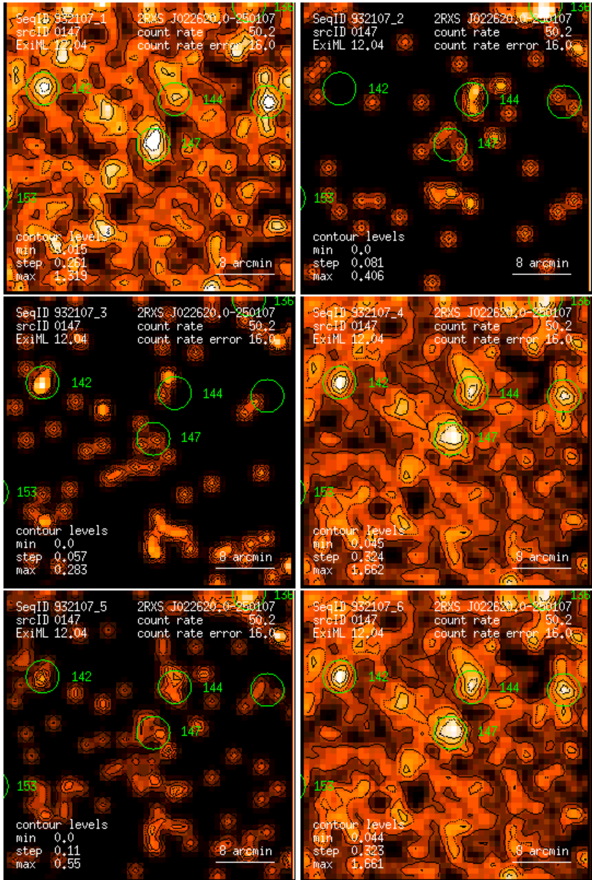
Figure 147: RASS 932107: detection 0147: band rate images, Gaussian filter: (1) PSPC channels 11 – 41, (2) 52 – 90, (3) 91 – 201, (4) 11 – 235, (5) 52 – 201, (6) 11 – 201. Broad band rates in counts/ks. Band rate contour levels in counts/ks/arcmin 2 .
