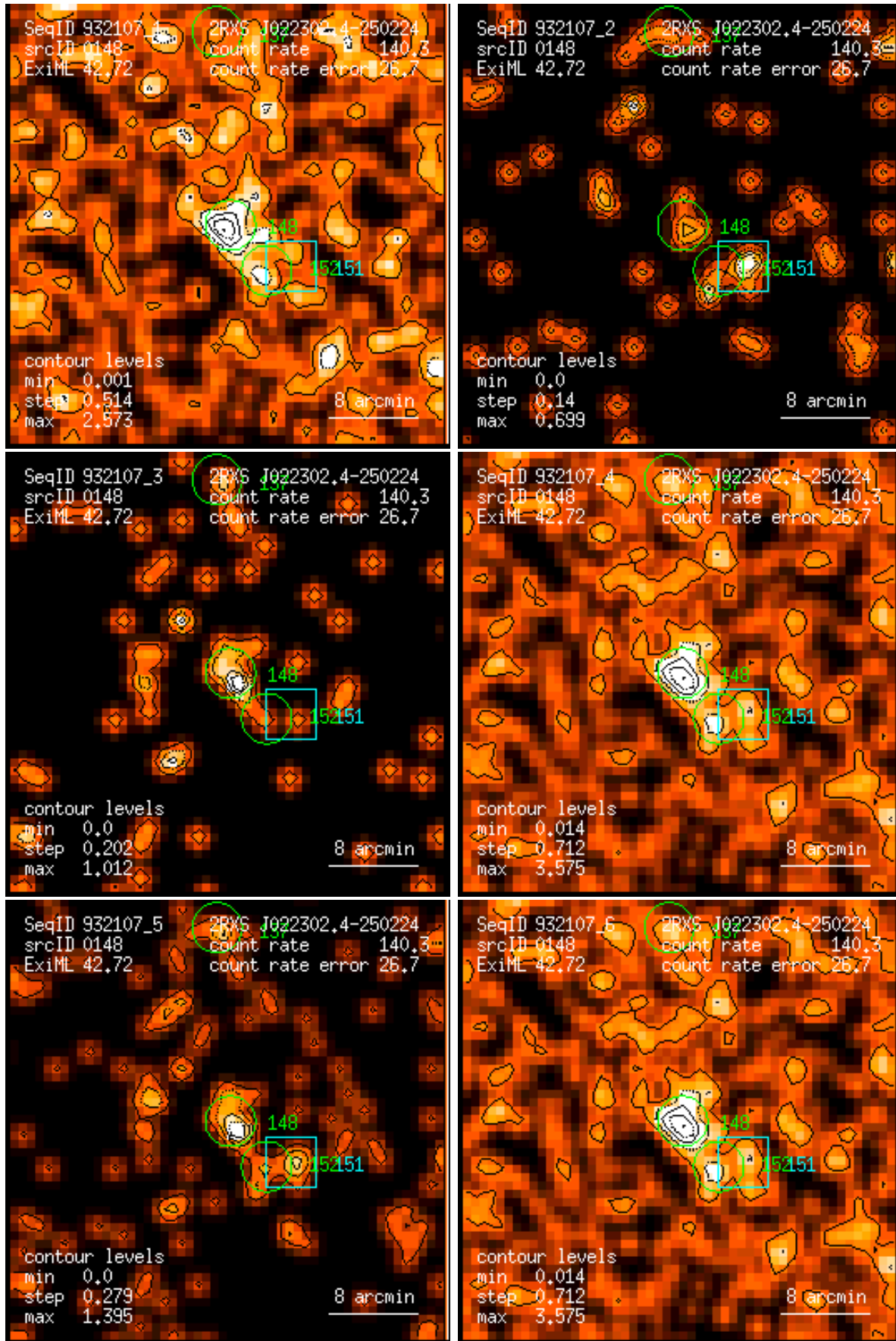
Figure 148: RASS 932107: detection 0148: band rate images, Gaussian filter: (1) PSPC channels 11 – 41, (2) 52 – 90, (3) 91 – 201, (4) 11 – 235, (5) 52 – 201, (6) 11 – 201. Broad band rates in counts/ks. Band rate contour levels in counts/ks/arcmin 2 .
