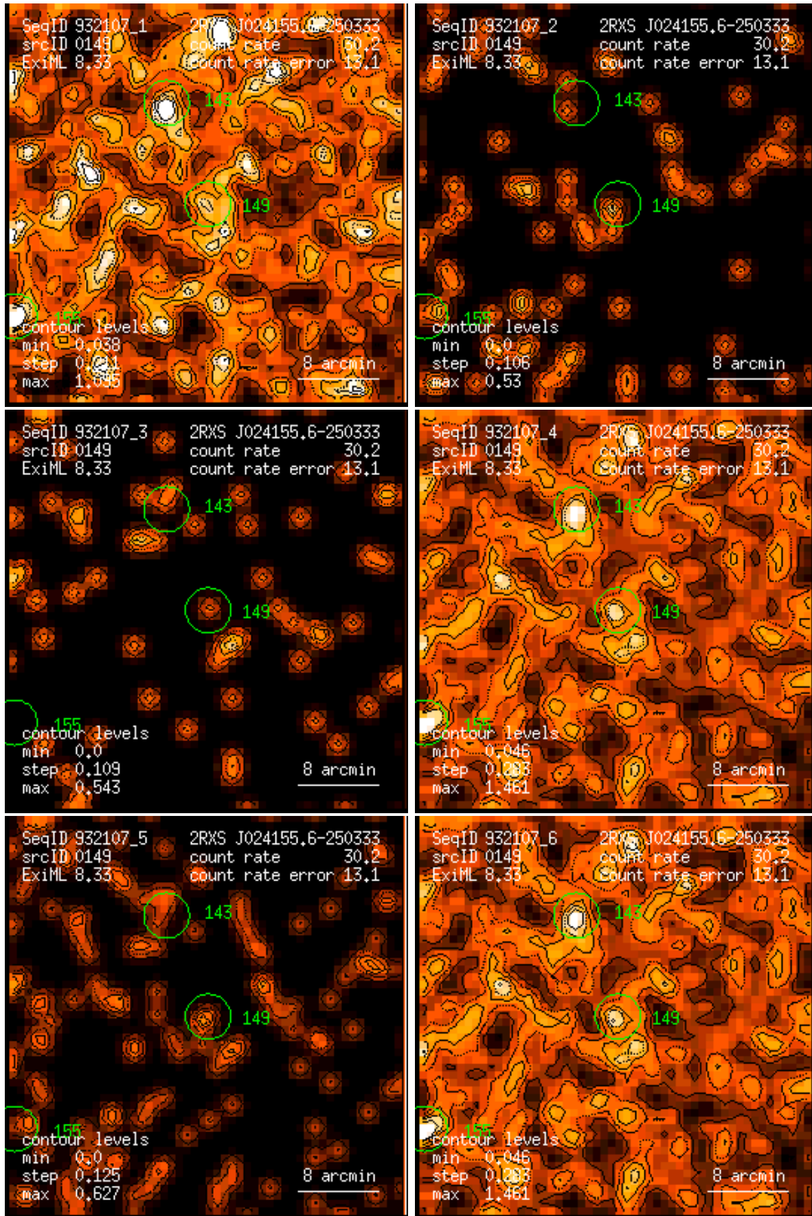
Figure 149: RASS 932107: detection 0149: band rate images, Gaussian filter: (1) PSPC channels 11 – 41, (2) 52 – 90, (3) 91 – 201, (4) 11 – 235, (5) 52 – 201, (6) 11 – 201. Broad band rates in counts/ks. Band rate contour levels in counts/ks/arcmin 2 .
