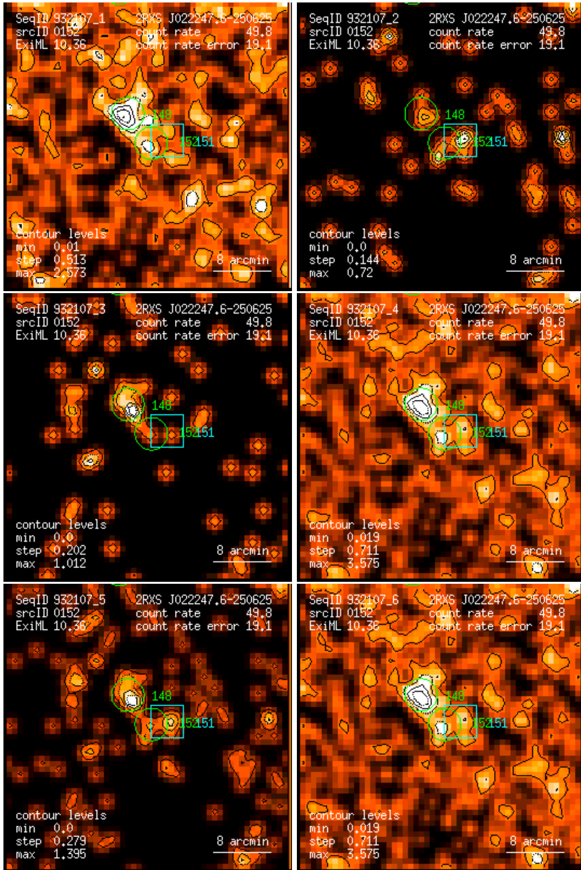
Figure 152: RASS 932107: detection 0152: band rate images, Gaussian filter: (1) PSPC channels 11 – 41, (2) 52 – 90, (3) 91 – 201, (4) 11 – 235, (5) 52 – 201, (6) 11 – 201. Broad band rates in counts/ks. Band rate contour levels in counts/ks/arcmin 2 .
