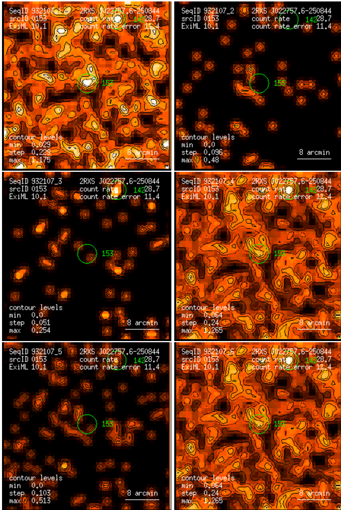
Figure 153: RASS 932107: detection 0153: band rate images, Gaussian filter: (1) PSPC channels 11 – 41, (2) 52 – 90, (3) 91 – 201, (4) 11 – 235, (5) 52 – 201, (6) 11 – 201. Broad band rates in counts/ks. Band rate contour levels in counts/ks/arcmin 2 .
