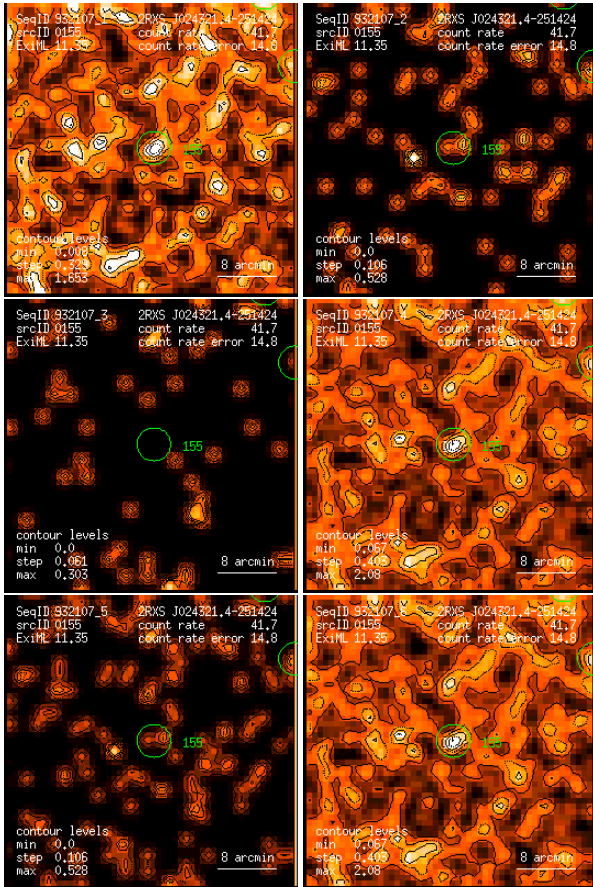
Figure 155: RASS 932107: detection 0155: band rate images, Gaussian filter: (1) PSPC channels 11 – 41, (2) 52 – 90, (3) 91 – 201, (4) 11 – 235, (5) 52 – 201, (6) 11 – 201. Broad band rates in counts/ks. Band rate contour levels in counts/ks/arcmin 2 .
