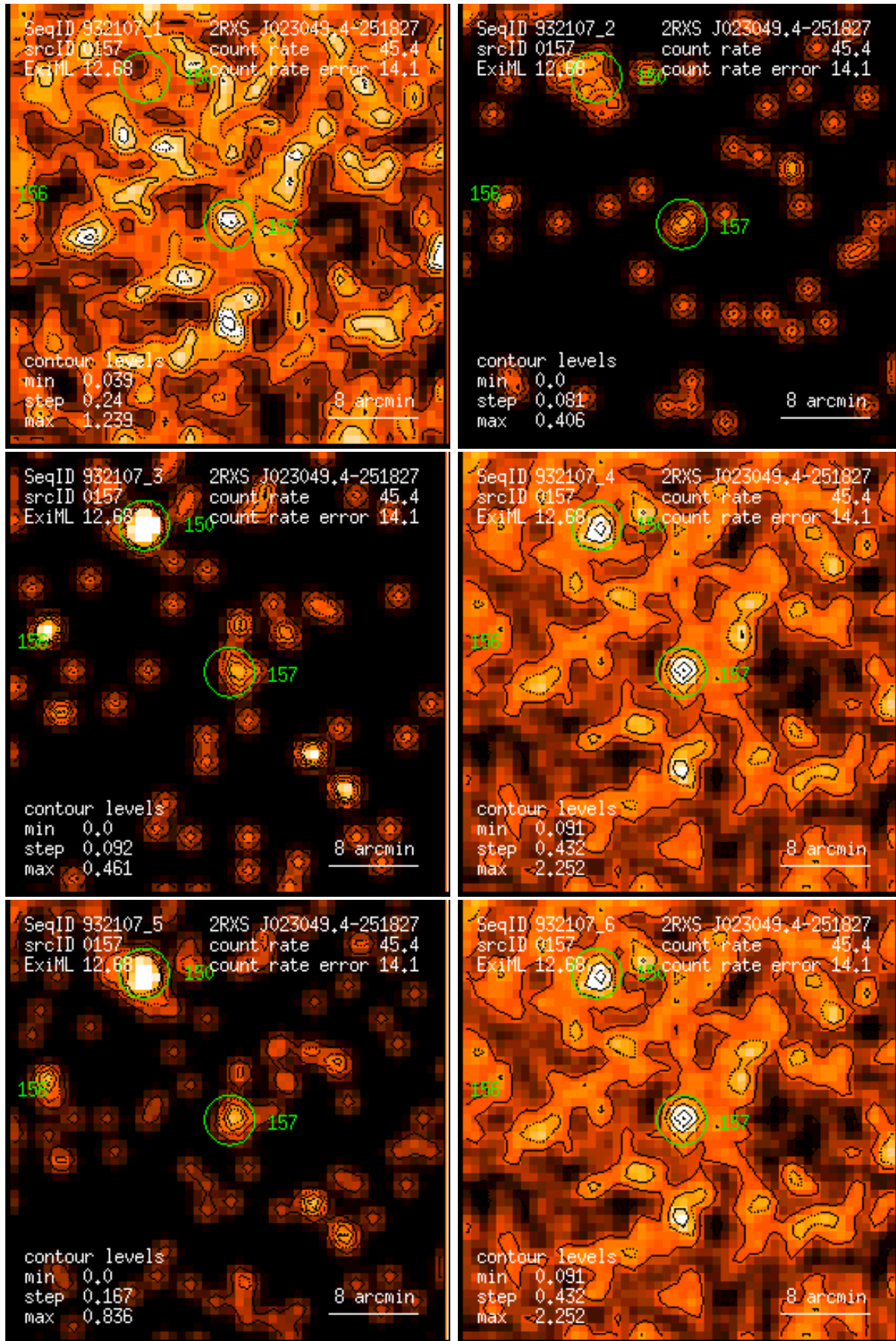
Figure 157: RASS 932107: detection 0157: band rate images, Gaussian filter: (1) PSPC channels 11 – 41, (2) 52 – 90, (3) 91 – 201, (4) 11 – 235, (5) 52 – 201, (6) 11 – 201. Broad band rates in counts/ks. Band rate contour levels in counts/ks/arcmin 2 .
