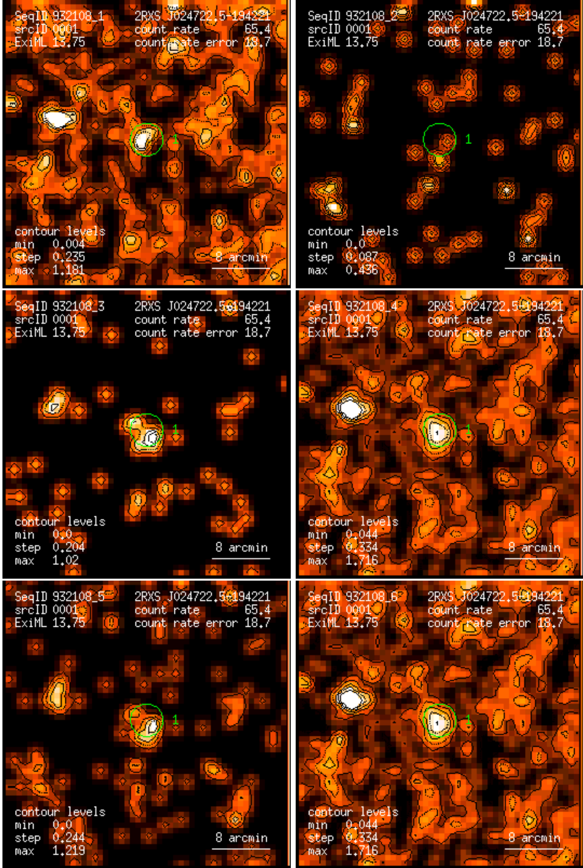
Figure 1: RASS 932108: detection 0001: band rate images, Gaussian filter: (1) PSPC channels 11 – 41, (2) 52 – 90, (3) 91 – 201, (4) 11 – 235, (5) 52 – 201, (6) 11 – 201. Broad band rates in counts/ks. Band rate contour levels in counts/ks/arcmin 2 .
