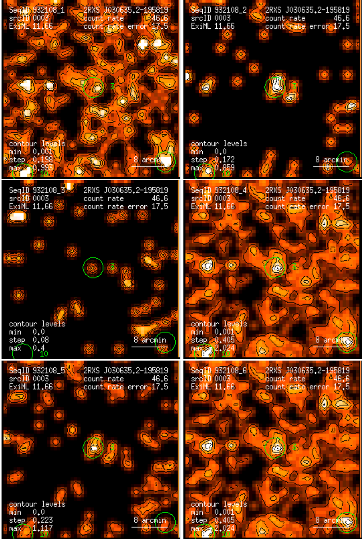
Figure 3: RASS 932108: detection 0003: band rate images, Gaussian filter: (1) PSPC channels 11 – 41, (2) 52 – 90, (3) 91 – 201, (4) 11 – 235, (5) 52 – 201, (6) 11 – 201. Broad band rates in counts/ks. Band rate contour levels in counts/ks/arcmin 2 .
