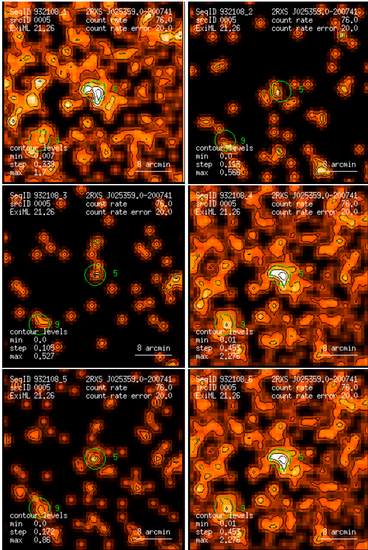
Figure 5: RASS 932108: detection 0005: band rate images, Gaussian filter: (1) PSPC channels 11 – 41, (2) 52 – 90, (3) 91 – 201, (4) 11 – 235, (5) 52 – 201, (6) 11 – 201. Broad band rates in counts/ks. Band rate contour levels in counts/ks/arcmin 2 .
