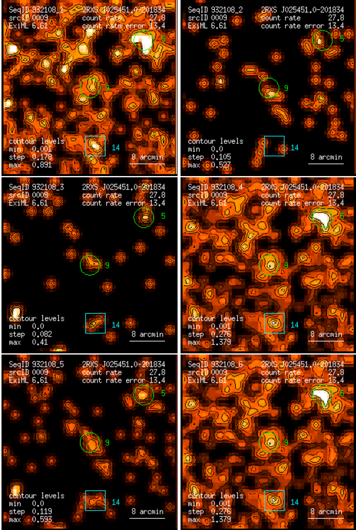
Figure 9: RASS 932108: detection 0009: band rate images, Gaussian filter: (1) PSPC channels 11 – 41, (2) 52 – 90, (3) 91 – 201, (4) 11 – 235, (5) 52 – 201, (6) 11 – 201. Broad band rates in counts/ks. Band rate contour levels in counts/ks/arcmin 2 .
