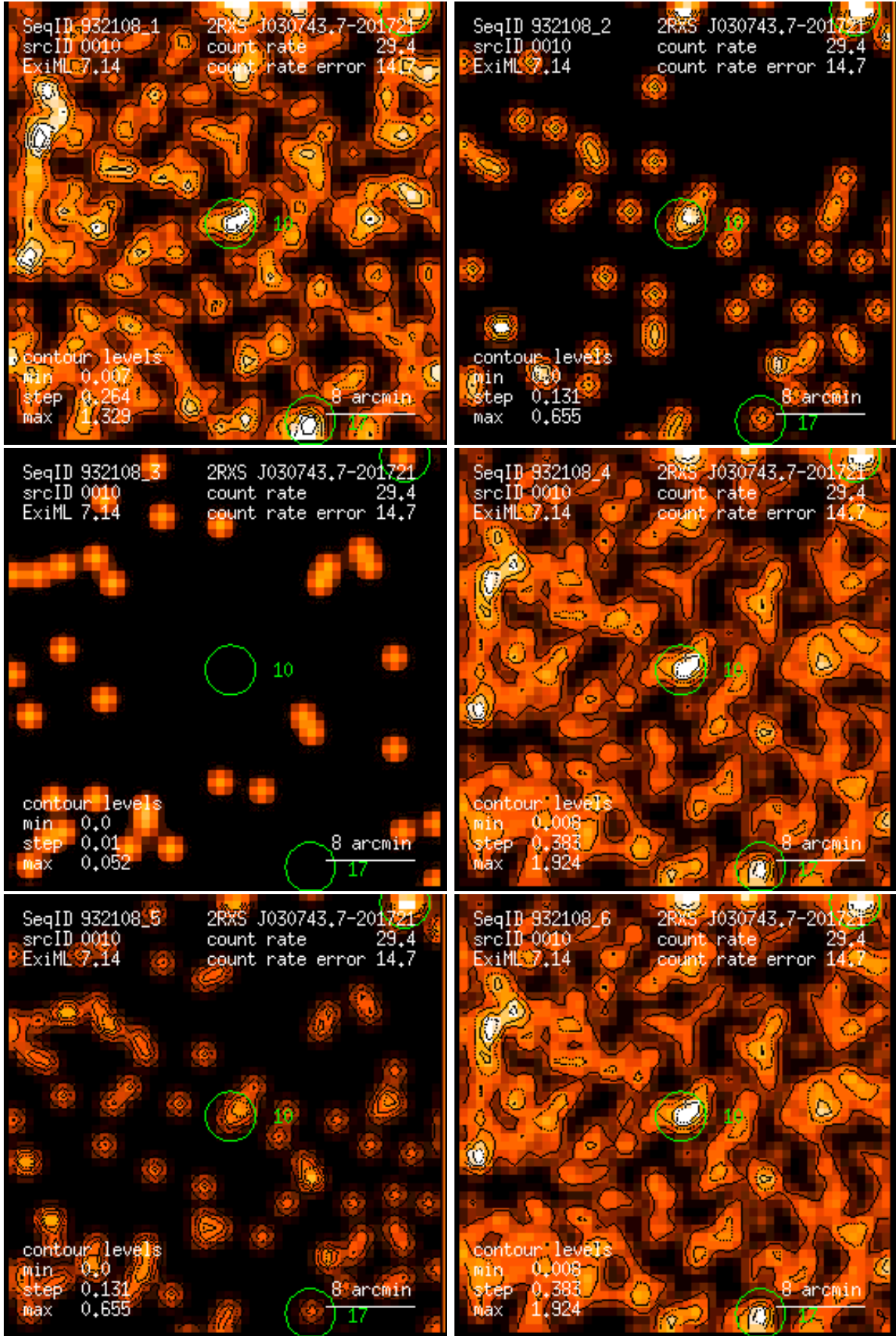
Figure 10: RASS 932108: detection 0010: band rate images, Gaussian filter: (1) PSPC channels 11 – 41, (2) 52 – 90, (3) 91 – 201, (4) 11 – 235, (5) 52 – 201, (6) 11 – 201. Broad band rates in counts/ks. Band rate contour levels in counts/ks/arcmin 2 .
