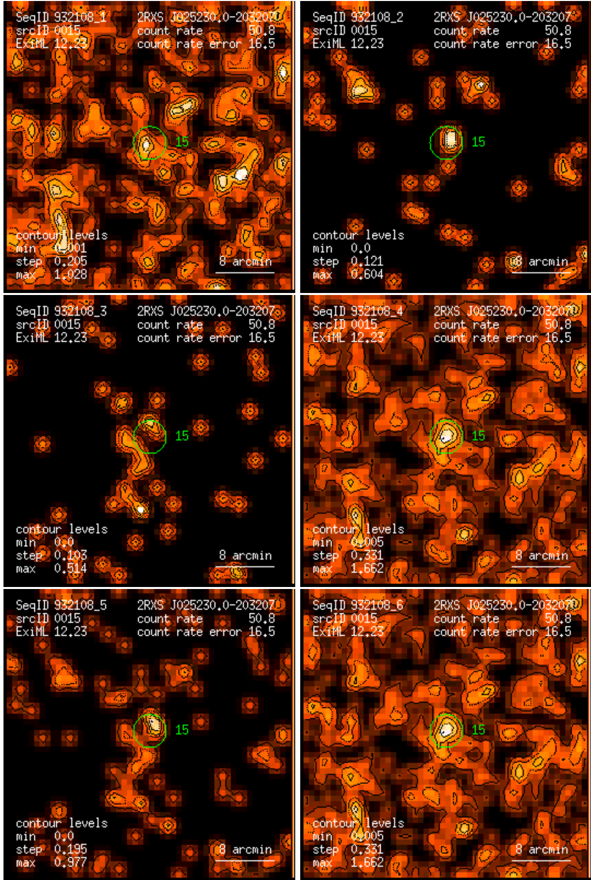
Figure 15: RASS 932108: detection 0015: band rate images, Gaussian filter: (1) PSPC channels 11 – 41, (2) 52 – 90, (3) 91 – 201, (4) 11 – 235, (5) 52 – 201, (6) 11 – 201. Broad band rates in counts/ks. Band rate contour levels in counts/ks/arcmin 2 .
