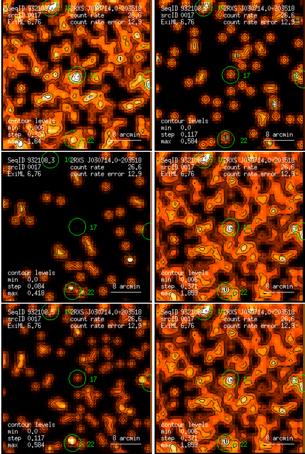
Figure 17: RASS 932108: detection 0017: band rate images, Gaussian filter: (1) PSPC channels 11 – 41, (2) 52 – 90, (3) 91 – 201, (4) 11 – 235, (5) 52 – 201, (6) 11 – 201. Broad band rates in counts/ks. Band rate contour levels in counts/ks/arcmin 2 .
