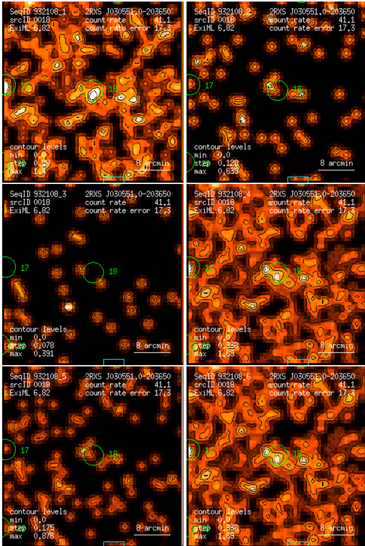
Figure 18: RASS 932108: detection 0018: band rate images, Gaussian filter: (1) PSPC channels 11 – 41, (2) 52 – 90, (3) 91 – 201, (4) 11 – 235, (5) 52 – 201, (6) 11 – 201. Broad band rates in counts/ks. Band rate contour levels in counts/ks/arcmin 2 .
