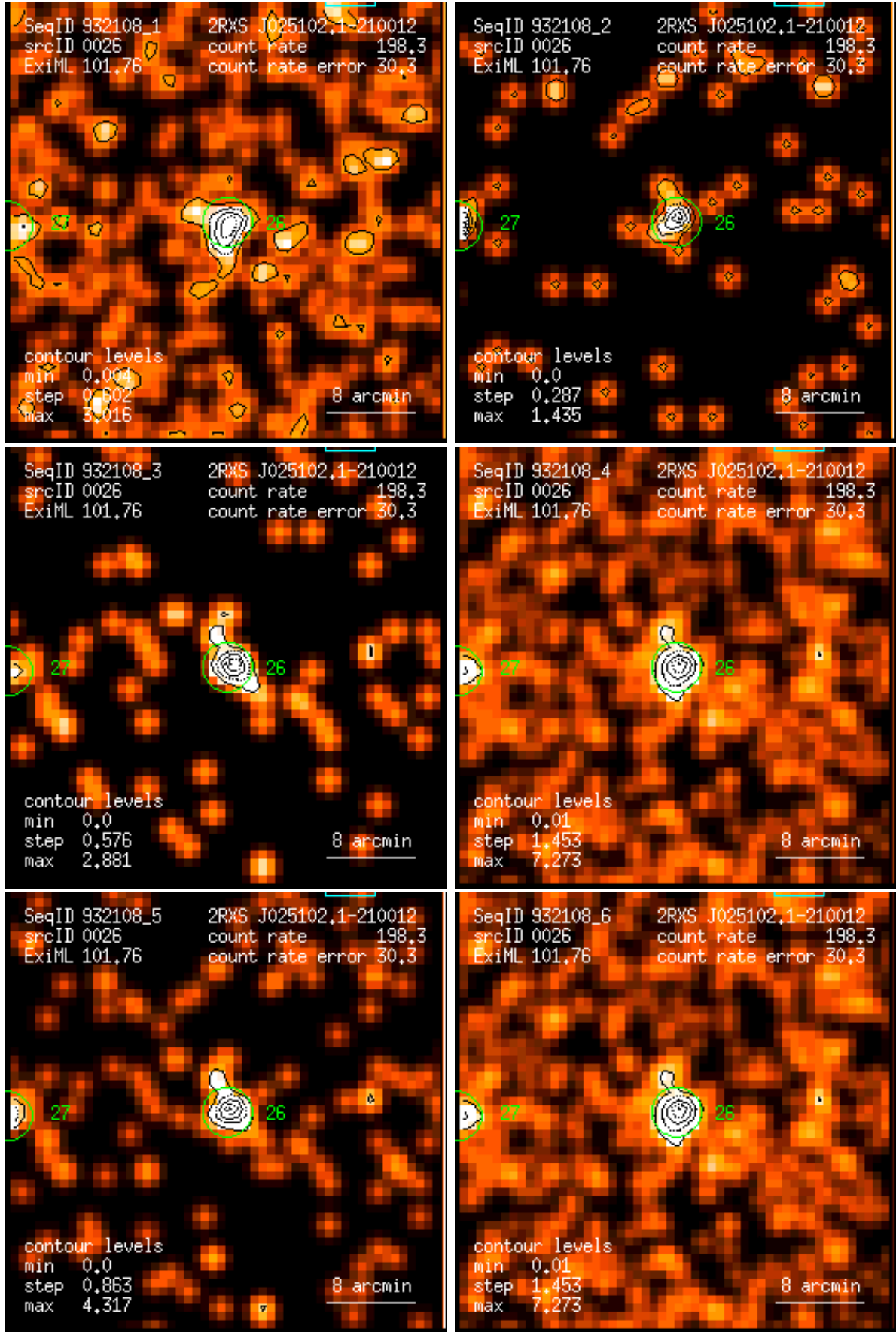
Figure 26: RASS 932108: detection 0026: band rate images, Gaussian filter: (1) PSPC channels 11 – 41, (2) 52 – 90, (3) 91 – 201, (4) 11 – 235, (5) 52 – 201, (6) 11 – 201. Broad band rates in counts/ks. Band rate contour levels in counts/ks/arcmin 2 .
