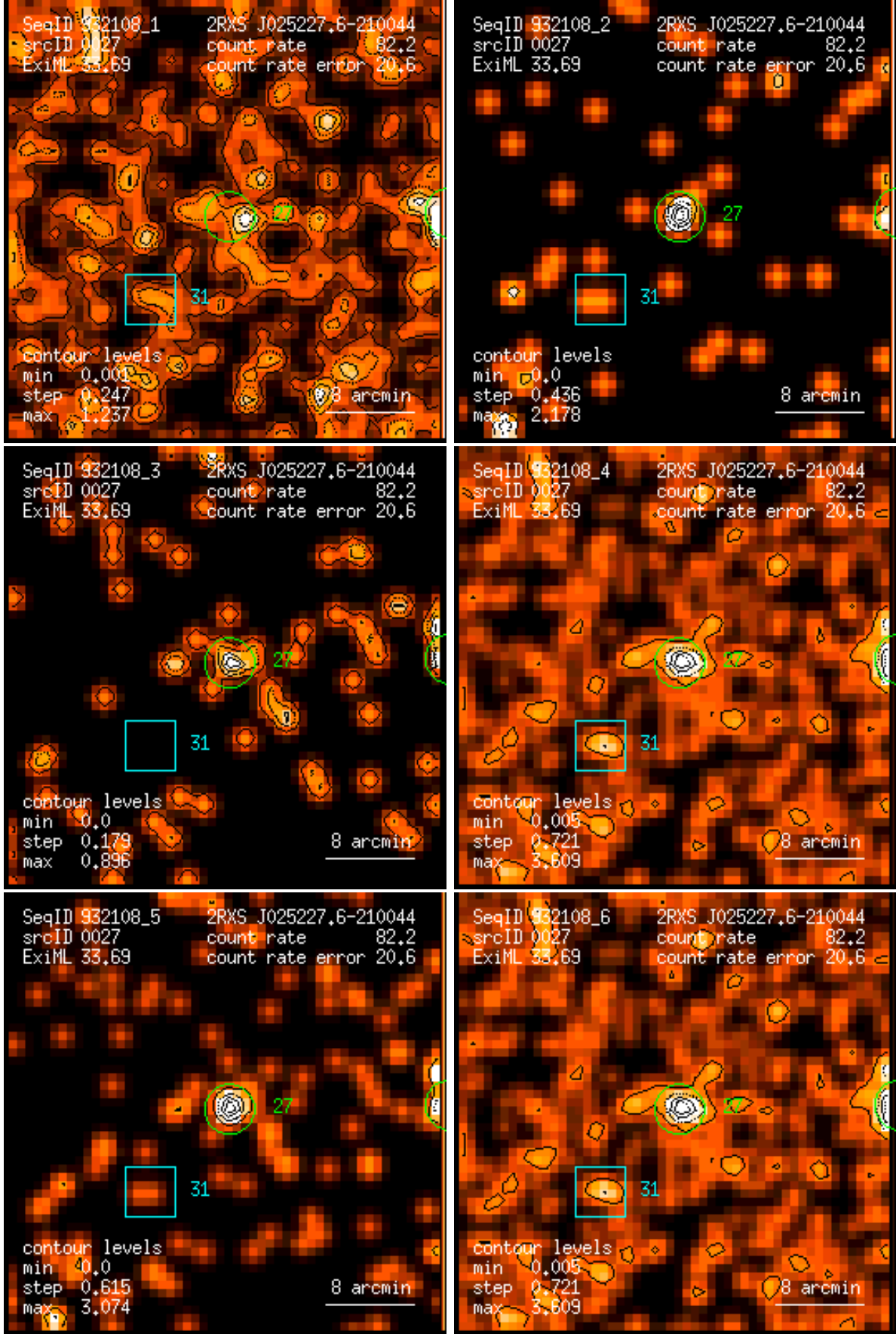
Figure 27: RASS 932108: detection 0027: band rate images, Gaussian filter: (1) PSPC channels 11 – 41, (2) 52 – 90, (3) 91 – 201, (4) 11 – 235, (5) 52 – 201, (6) 11 – 201. Broad band rates in counts/ks. Band rate contour levels in counts/ks/arcmin 2 .
