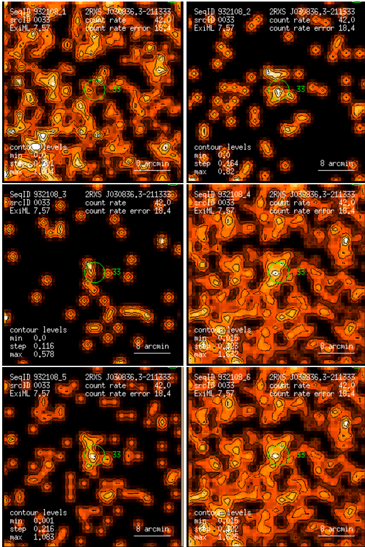
Figure 33: RASS 932108: detection 0033: band rate images, Gaussian filter: (1) PSPC channels 11 – 41, (2) 52 – 90, (3) 91 – 201, (4) 11 – 235, (5) 52 – 201, (6) 11 – 201. Broad band rates in counts/ks. Band rate contour levels in counts/ks/arcmin 2 .
