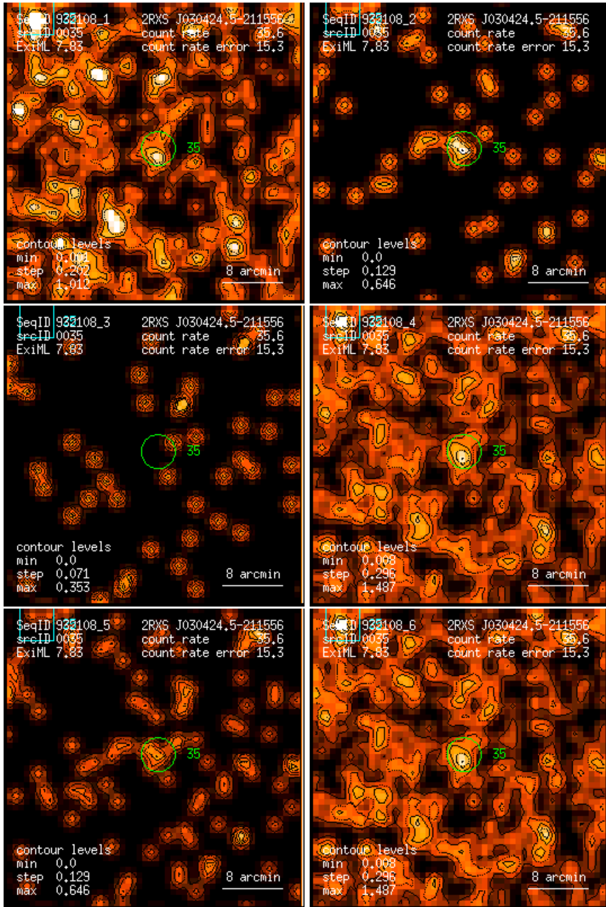
Figure 35: RASS 932108: detection 0035: band rate images, Gaussian filter: (1) PSPC channels 11 – 41, (2) 52 – 90, (3) 91 – 201, (4) 11 – 235, (5) 52 – 201, (6) 11 – 201. Broad band rates in counts/ks. Band rate contour levels in counts/ks/arcmin 2 .
