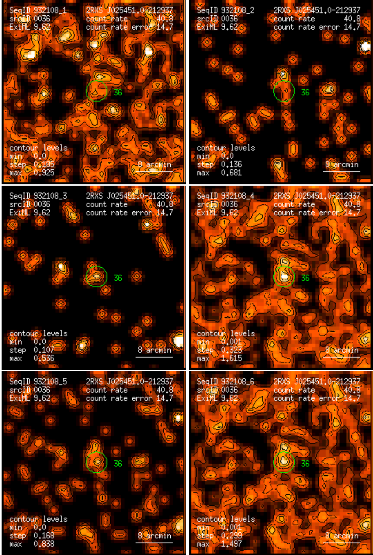
Figure 36: RASS 932108: detection 0036: band rate images, Gaussian filter: (1) PSPC channels 11 – 41, (2) 52 – 90, (3) 91 – 201, (4) 11 – 235, (5) 52 – 201, (6) 11 – 201. Broad band rates in counts/ks. Band rate contour levels in counts/ks/arcmin 2 .
