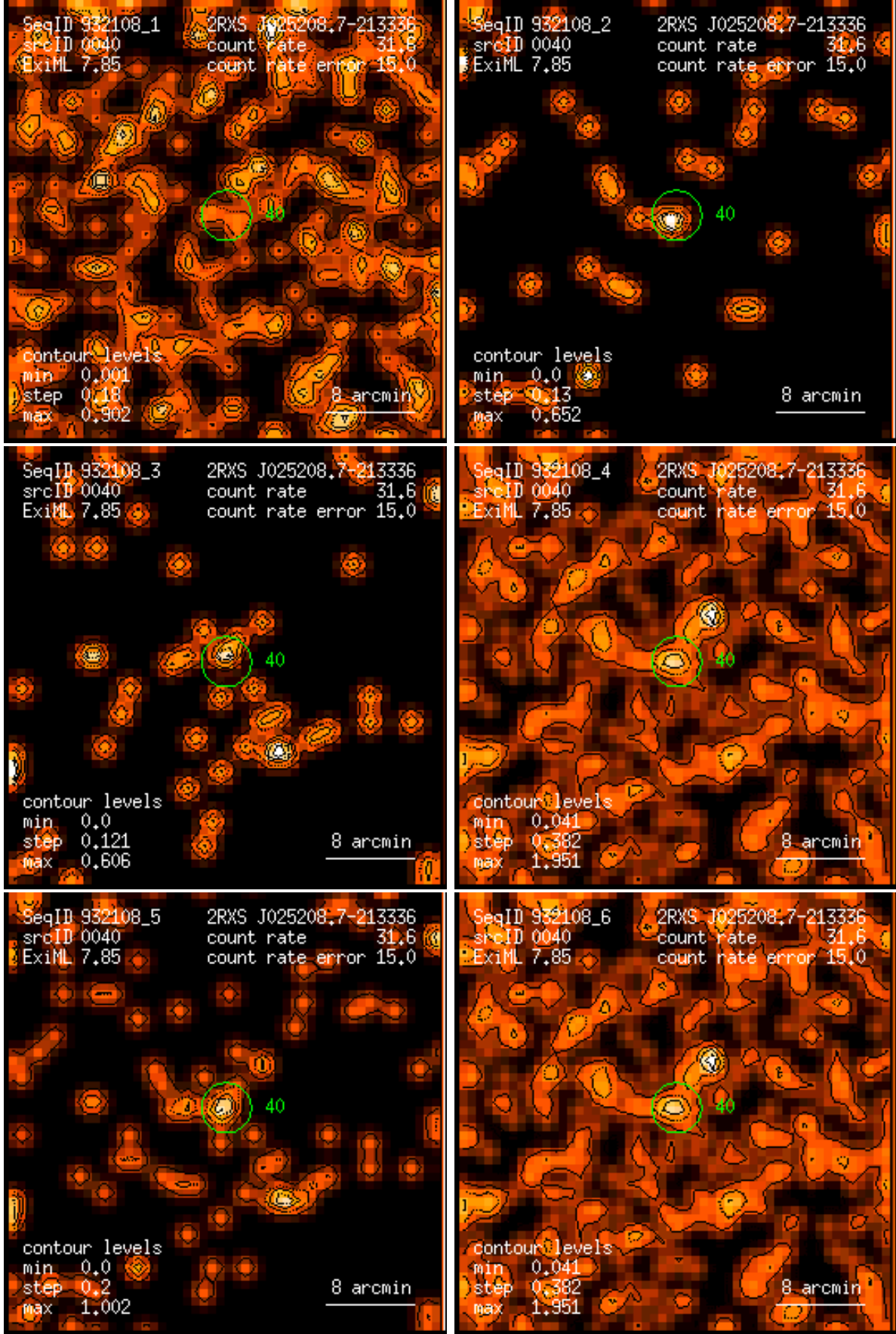
Figure 40: RASS 932108: detection 0040: band rate images, Gaussian filter: (1) PSPC channels 11 – 41, (2) 52 – 90, (3) 91 – 201, (4) 11 – 235, (5) 52 – 201, (6) 11 – 201. Broad band rates in counts/ks. Band rate contour levels in counts/ks/arcmin 2 .
