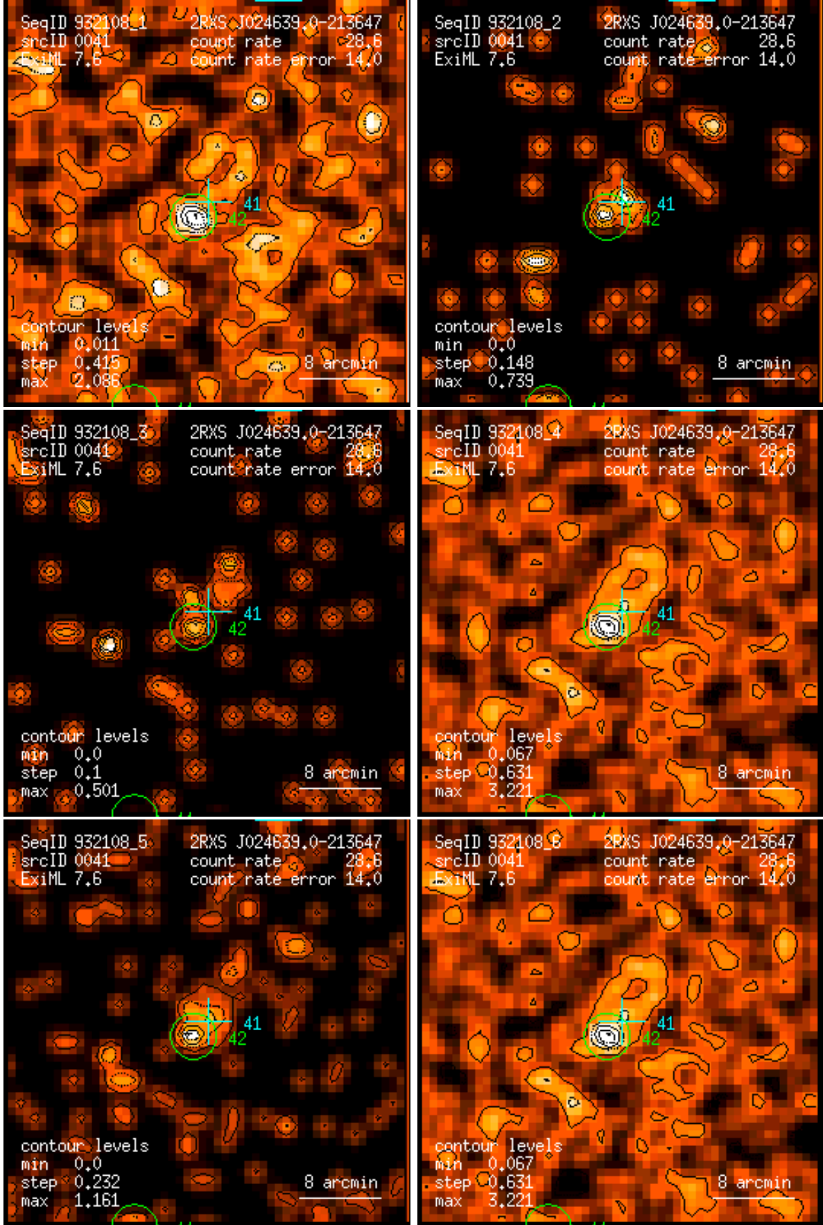
Figure 41: RASS 932108: detection 0041: band rate images, Gaussian filter: (1) PSPC channels 11 – 41, (2) 52 – 90, (3) 91 – 201, (4) 11 – 235, (5) 52 – 201, (6) 11 – 201. Broad band rates in counts/ks. Band rate contour levels in counts/ks/arcmin 2 .
