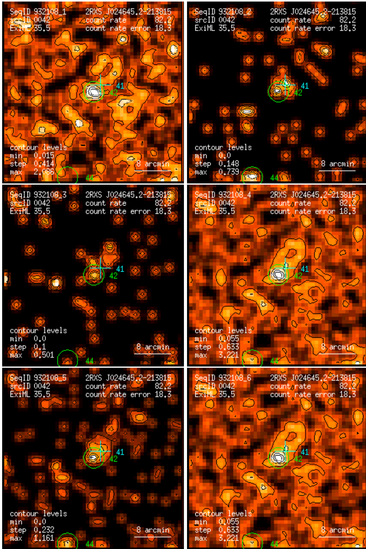
Figure 42: RASS 932108: detection 0042: band rate images, Gaussian filter: (1) PSPC channels 11 – 41, (2) 52 – 90, (3) 91 – 201, (4) 11 – 235, (5) 52 – 201, (6) 11 – 201. Broad band rates in counts/ks. Band rate contour levels in counts/ks/arcmin 2 .
