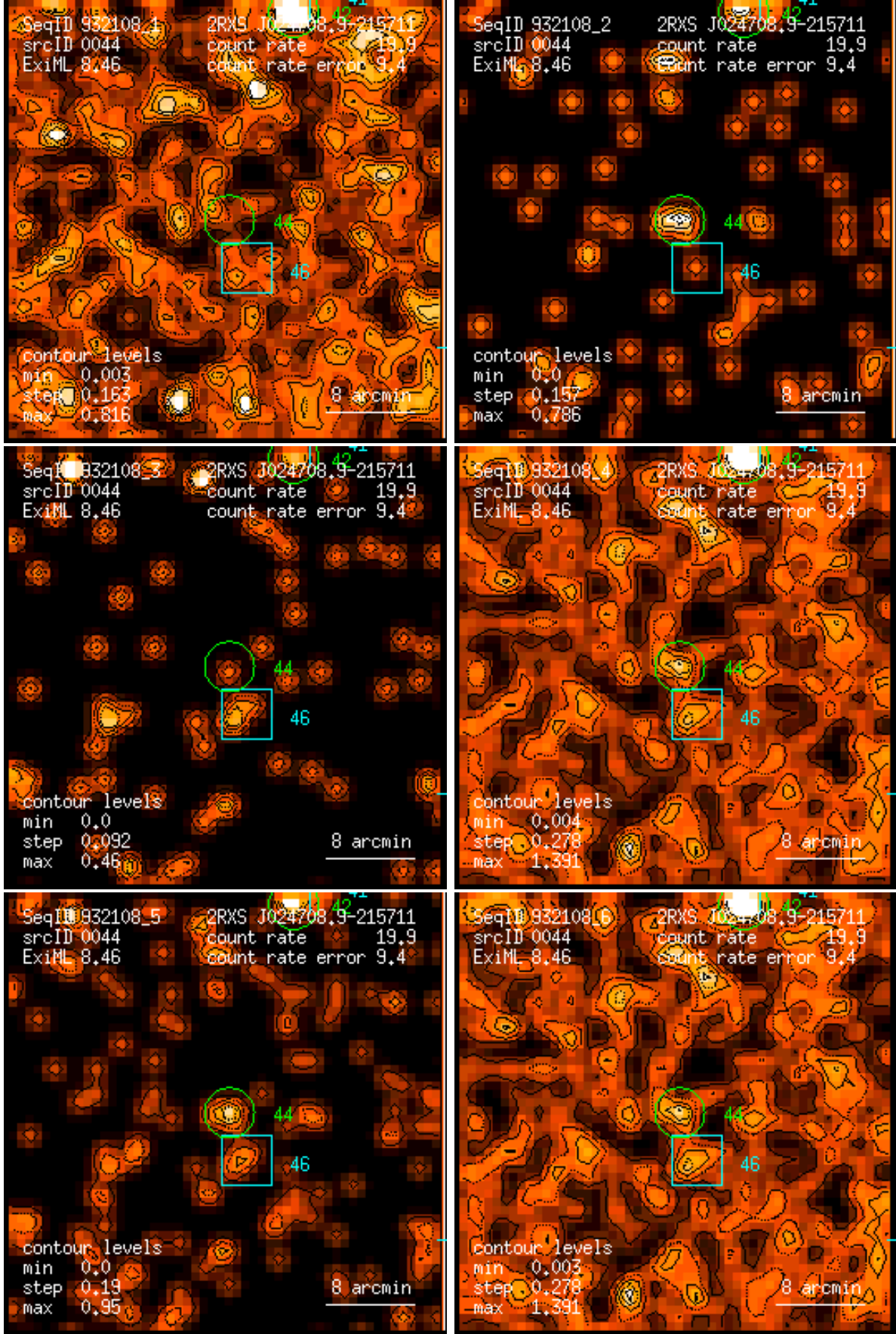
Figure 44: RASS 932108: detection 0044: band rate images, Gaussian filter: (1) PSPC channels 11 – 41, (2) 52 – 90, (3) 91 – 201, (4) 11 – 235, (5) 52 – 201, (6) 11 – 201. Broad band rates in counts/ks. Band rate contour levels in counts/ks/arcmin 2 .
