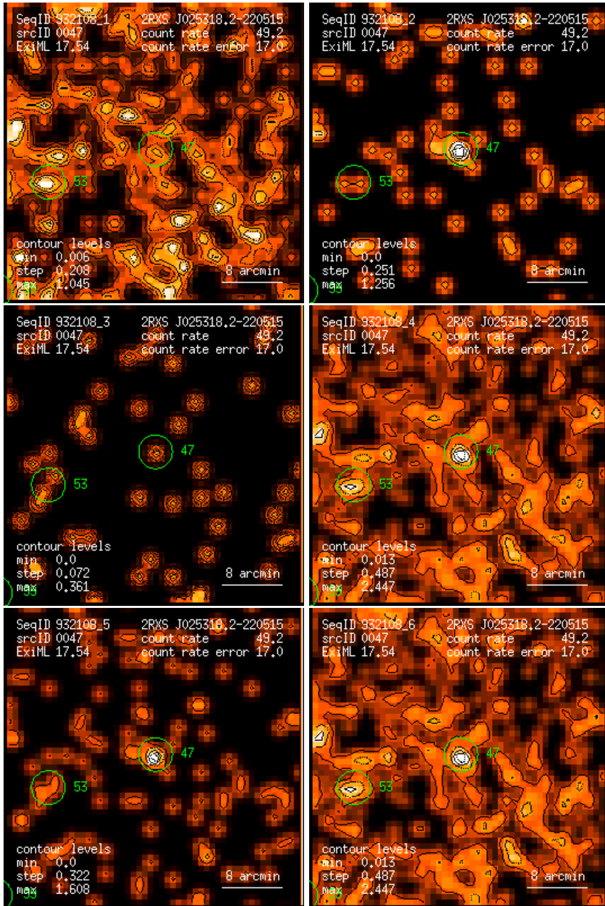
Figure 47: RASS 932108: detection 0047: band rate images, Gaussian filter: (1) PSPC channels 11 – 41, (2) 52 – 90, (3) 91 – 201, (4) 11 – 235, (5) 52 – 201, (6) 11 – 201. Broad band rates in counts/ks. Band rate contour levels in counts/ks/arcmin 2 .
