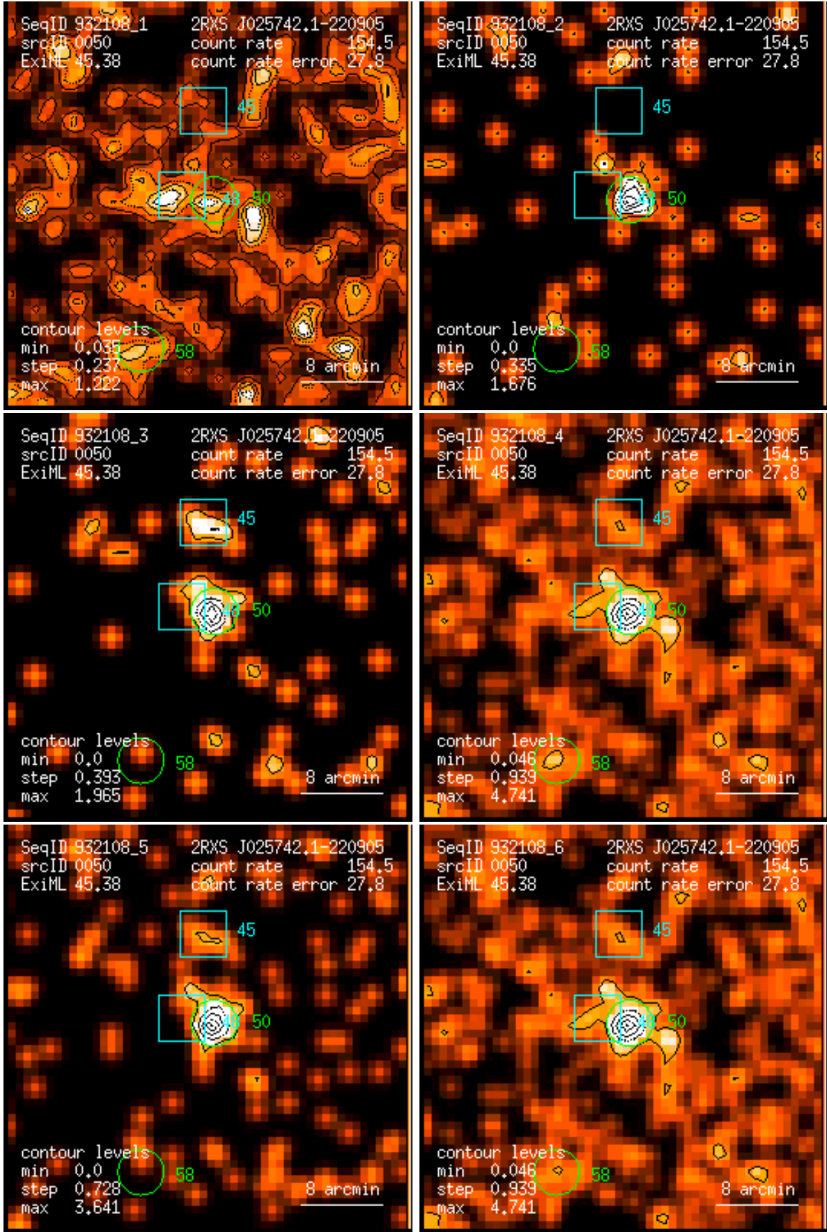
Figure 50: RASS 932108: detection 0050: band rate images, Gaussian filter: (1) PSPC channels 11 – 41, (2) 52 – 90, (3) 91 – 201, (4) 11 – 235, (5) 52 – 201, (6) 11 – 201. Broad band rates in counts/ks. Band rate contour levels in counts/ks/arcmin 2 .
