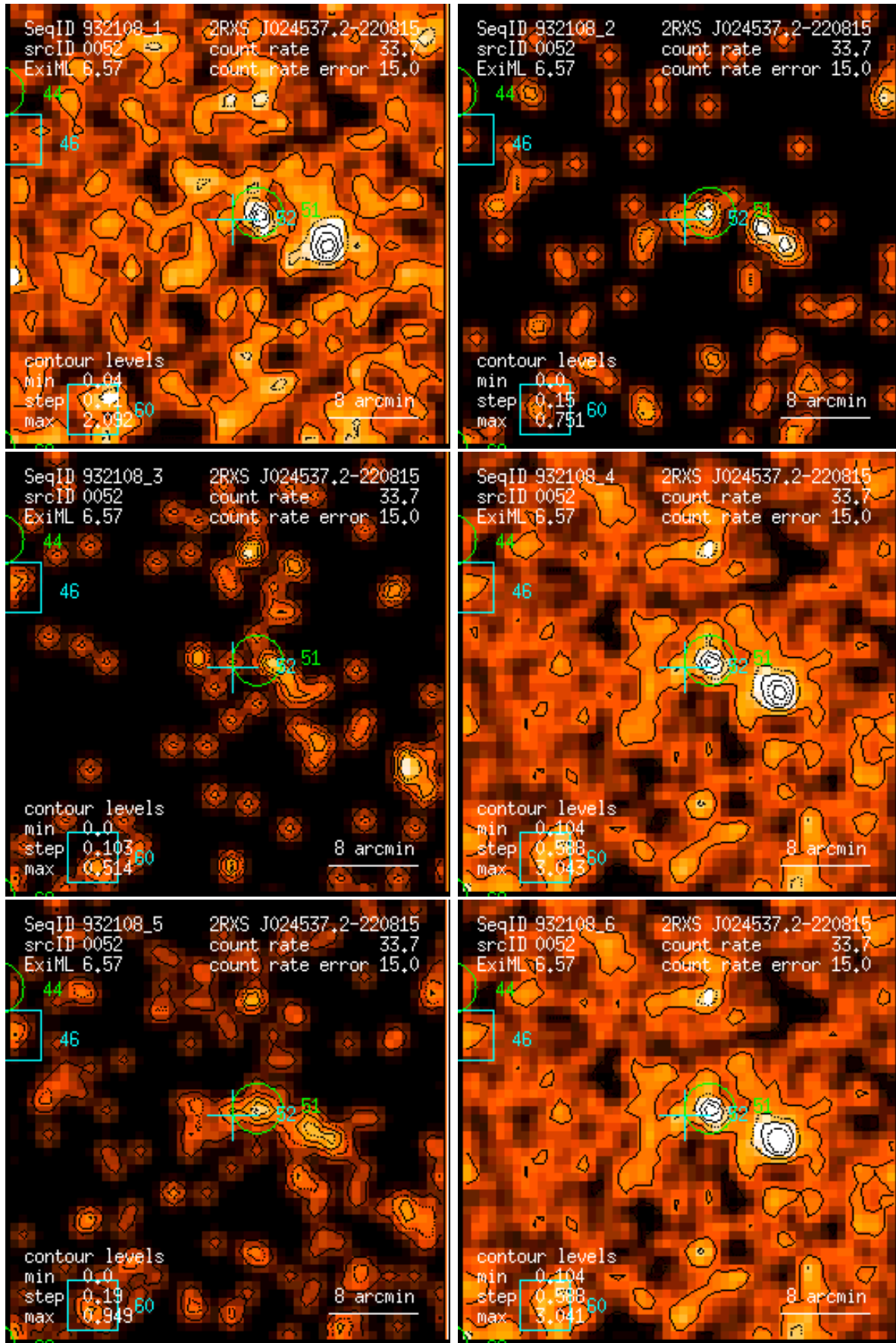
Figure 52: RASS 932108: detection 0052: band rate images, Gaussian filter: (1) PSPC channels 11 – 41, (2) 52 – 90, (3) 91 – 201, (4) 11 – 235, (5) 52 – 201, (6) 11 – 201. Broad band rates in counts/ks. Band rate contour levels in counts/ks/arcmin 2 .
