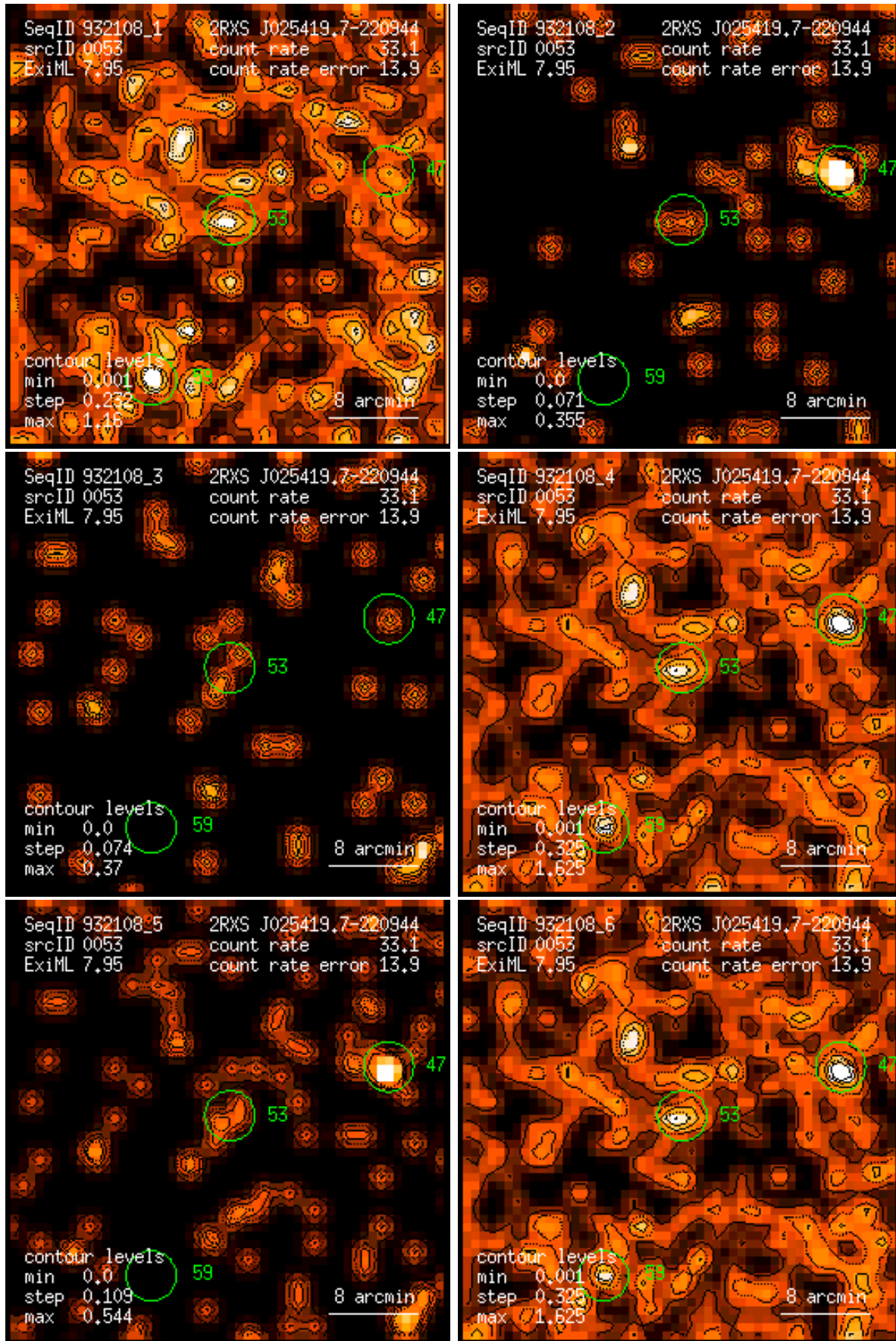
Figure 53: RASS 932108: detection 0053: band rate images, Gaussian filter: (1) PSPC channels 11 – 41, (2) 52 – 90, (3) 91 – 201, (4) 11 – 235, (5) 52 – 201, (6) 11 – 201. Broad band rates in counts/ks. Band rate contour levels in counts/ks/arcmin 2 .
