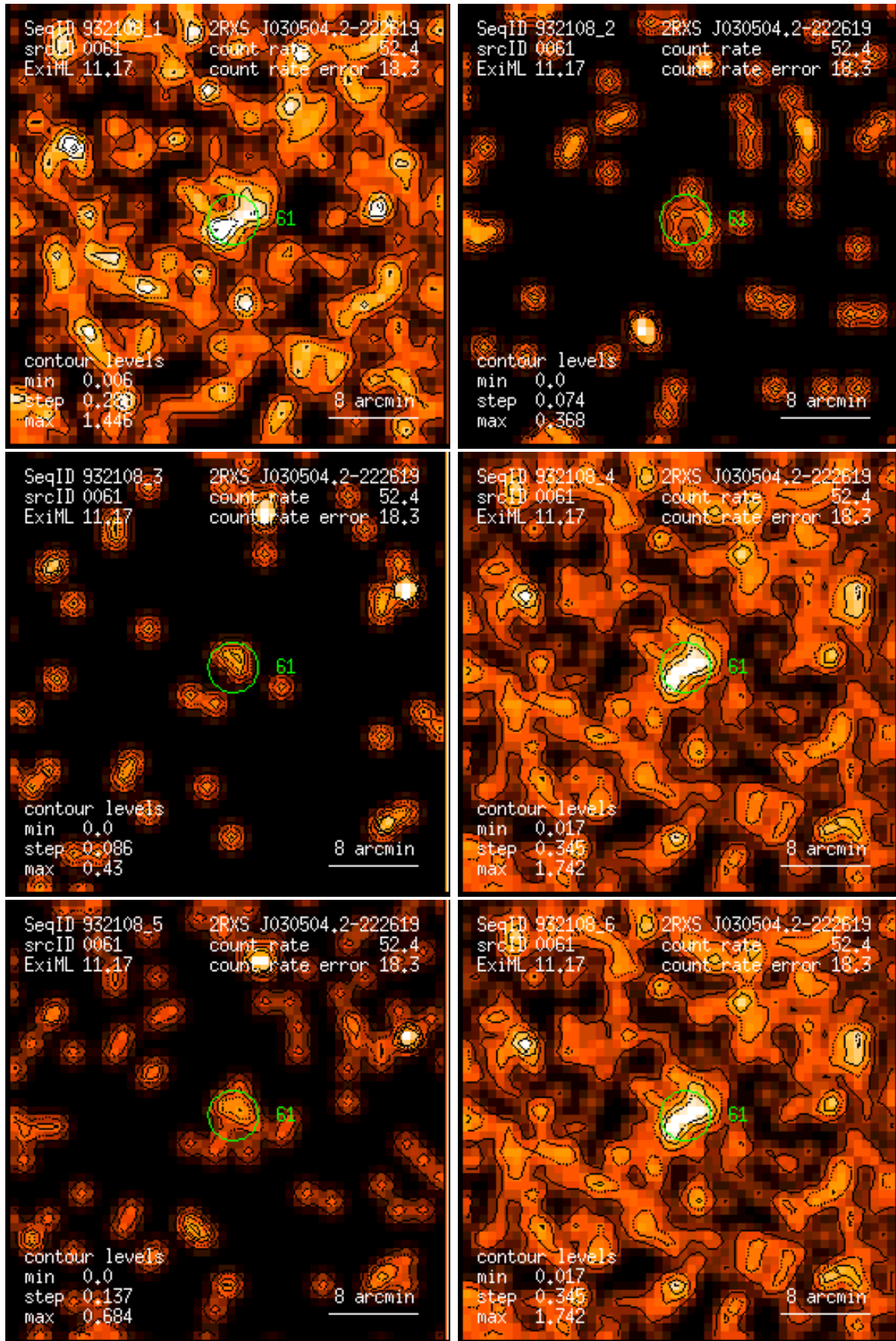
Figure 61: RASS 932108: detection 0061: band rate images, Gaussian filter: (1) PSPC channels 11 – 41, (2) 52 – 90, (3) 91 – 201, (4) 11 – 235, (5) 52 – 201, (6) 11 – 201. Broad band rates in counts/ks. Band rate contour levels in counts/ks/arcmin 2 .
