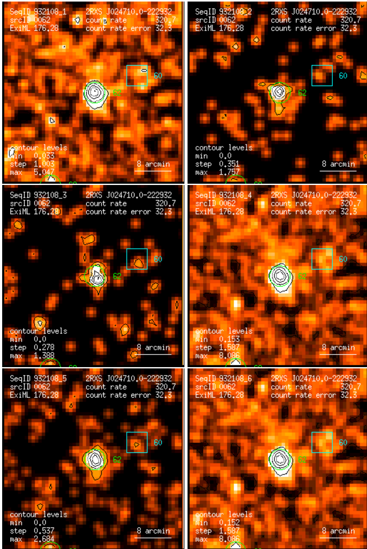
Figure 62: RASS 932108: detection 0062: band rate images, Gaussian filter: (1) PSPC channels 11 – 41, (2) 52 – 90, (3) 91 – 201, (4) 11 – 235, (5) 52 – 201, (6) 11 – 201. Broad band rates in counts/ks. Band rate contour levels in counts/ks/arcmin 2 .
