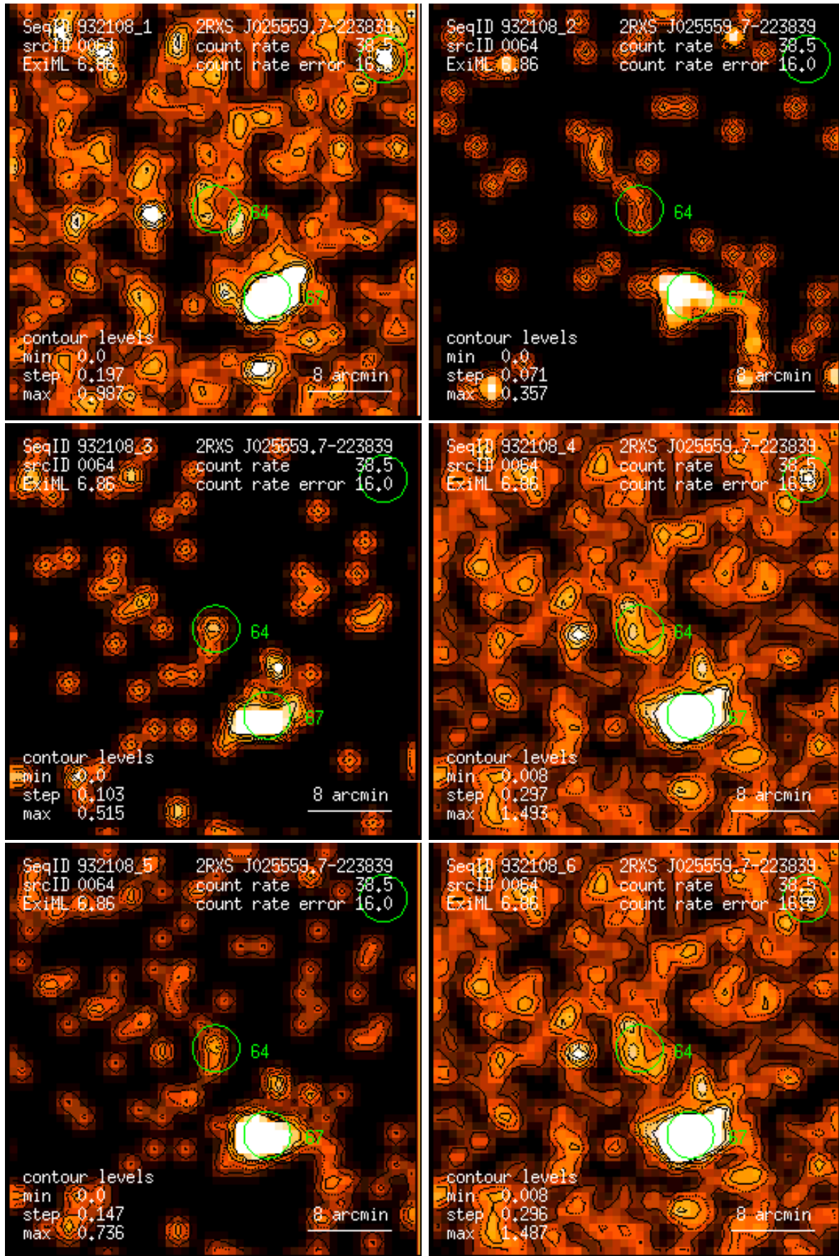
Figure 64: RASS 932108: detection 0064: band rate images, Gaussian filter: (1) PSPC channels 11 – 41, (2) 52 – 90, (3) 91 – 201, (4) 11 – 235, (5) 52 – 201, (6) 11 – 201. Broad band rates in counts/ks. Band rate contour levels in counts/ks/arcmin 2 .
