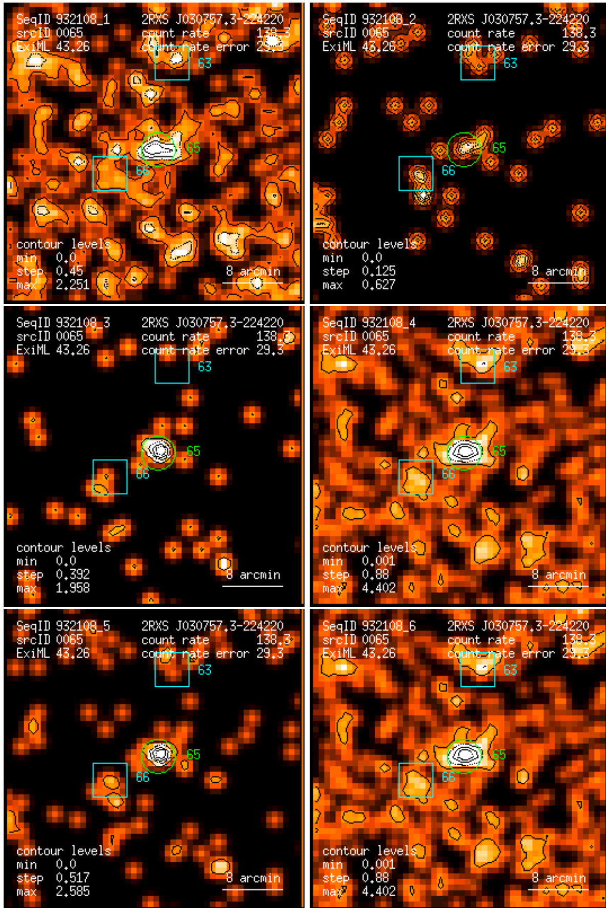
Figure 65: RASS 932108: detection 0065: band rate images, Gaussian filter: (1) PSPC channels 11 – 41, (2) 52 – 90, (3) 91 – 201, (4) 11 – 235, (5) 52 – 201, (6) 11 – 201. Broad band rates in counts/ks. Band rate contour levels in counts/ks/arcmin 2 .
