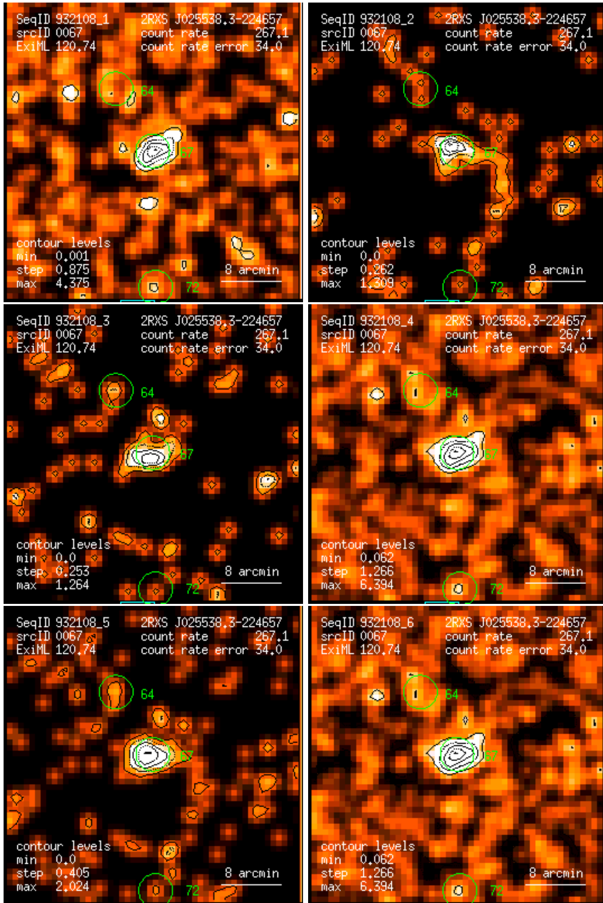
Figure 67: RASS 932108: detection 0067: band rate images, Gaussian filter: (1) PSPC channels 11 – 41, (2) 52 – 90, (3) 91 – 201, (4) 11 – 235, (5) 52 – 201, (6) 11 – 201. Broad band rates in counts/ks. Band rate contour levels in counts/ks/arcmin 2 .
