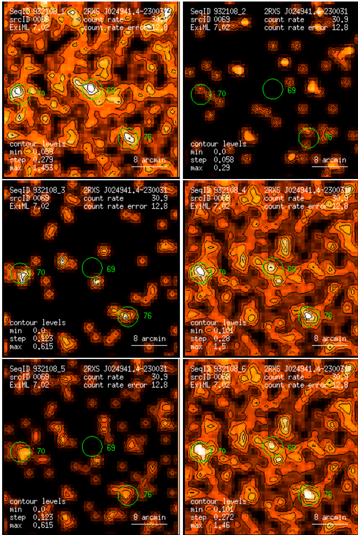
Figure 69: RASS 932108: detection 0069: band rate images, Gaussian filter: (1) PSPC channels 11 – 41, (2) 52 – 90, (3) 91 – 201, (4) 11 – 235, (5) 52 – 201, (6) 11 – 201. Broad band rates in counts/ks. Band rate contour levels in counts/ks/arcmin 2 .
