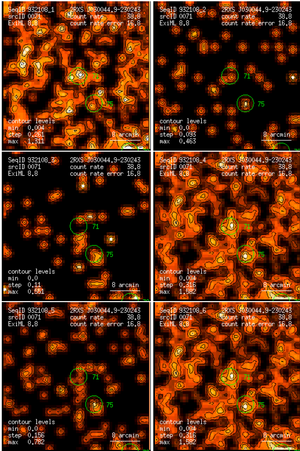
Figure 71: RASS 932108: detection 0071: band rate images, Gaussian filter: (1) PSPC channels 11 – 41, (2) 52 – 90, (3) 91 – 201, (4) 11 – 235, (5) 52 – 201, (6) 11 – 201. Broad band rates in counts/ks. Band rate contour levels in counts/ks/arcmin 2 .
