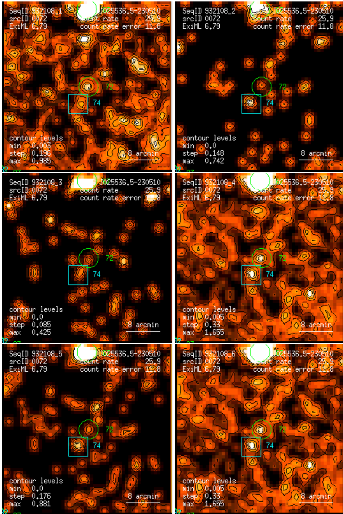
Figure 72: RASS 932108: detection 0072: band rate images, Gaussian filter: (1) PSPC channels 11 – 41, (2) 52 – 90, (3) 91 – 201, (4) 11 – 235, (5) 52 – 201, (6) 11 – 201. Broad band rates in counts/ks. Band rate contour levels in counts/ks/arcmin 2 .
