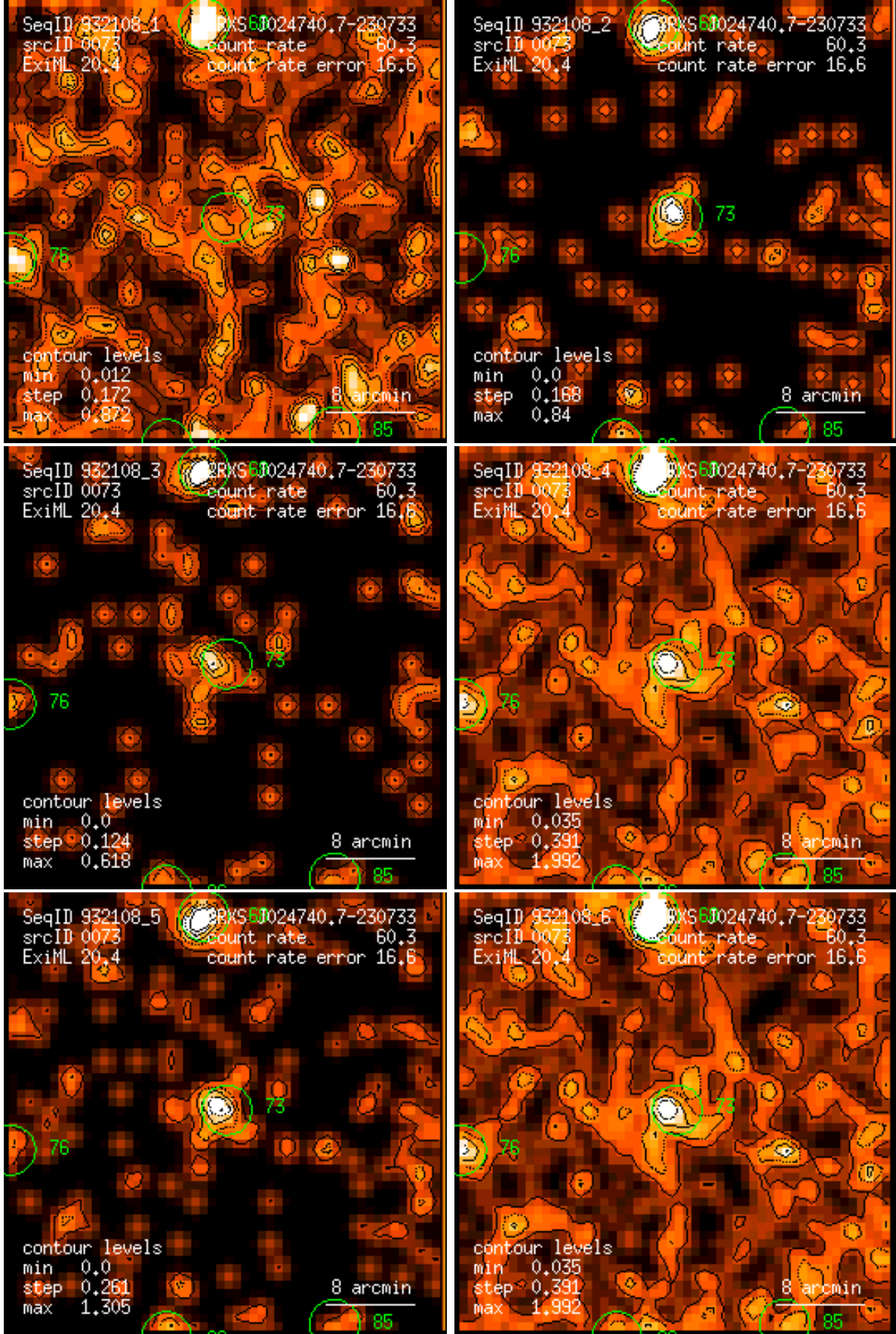
Figure 73: RASS 932108: detection 0073: band rate images, Gaussian filter: (1) PSPC channels 11 – 41, (2) 52 – 90, (3) 91 – 201, (4) 11 – 235, (5) 52 – 201, (6) 11 – 201. Broad band rates in counts/ks. Band rate contour levels in counts/ks/arcmin 2 .
