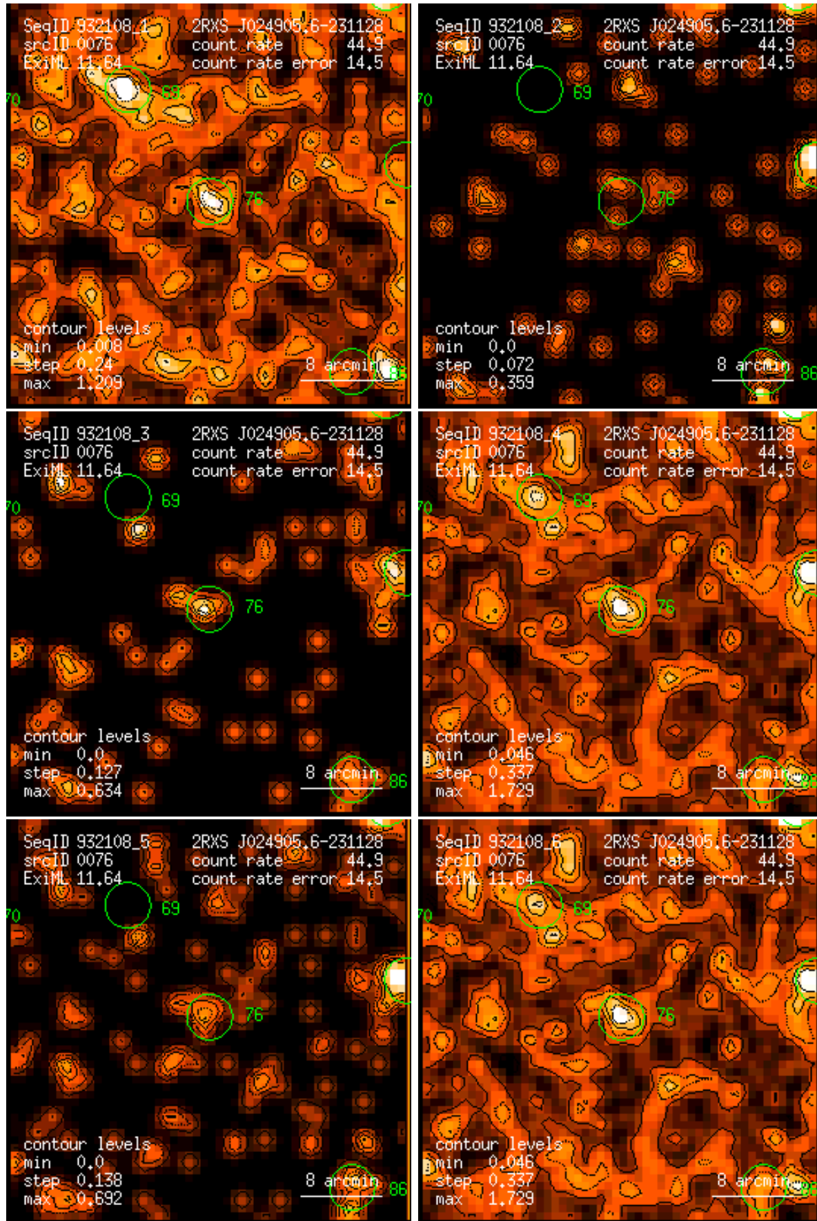
Figure 76: RASS 932108: detection 0076: band rate images, Gaussian filter: (1) PSPC channels 11 – 41, (2) 52 – 90, (3) 91 – 201, (4) 11 – 235, (5) 52 – 201, (6) 11 – 201. Broad band rates in counts/ks. Band rate contour levels in counts/ks/arcmin 2 .
