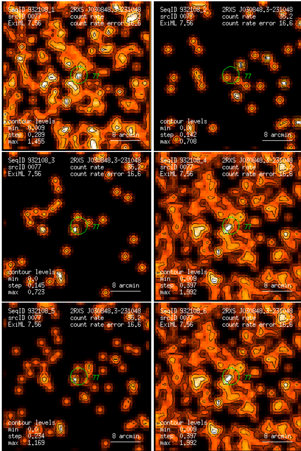
Figure 77: RASS 932108: detection 0077: band rate images, Gaussian filter: (1) PSPC channels 11 – 41, (2) 52 – 90, (3) 91 – 201, (4) 11 – 235, (5) 52 – 201, (6) 11 – 201. Broad band rates in counts/ks. Band rate contour levels in counts/ks/arcmin 2 .
