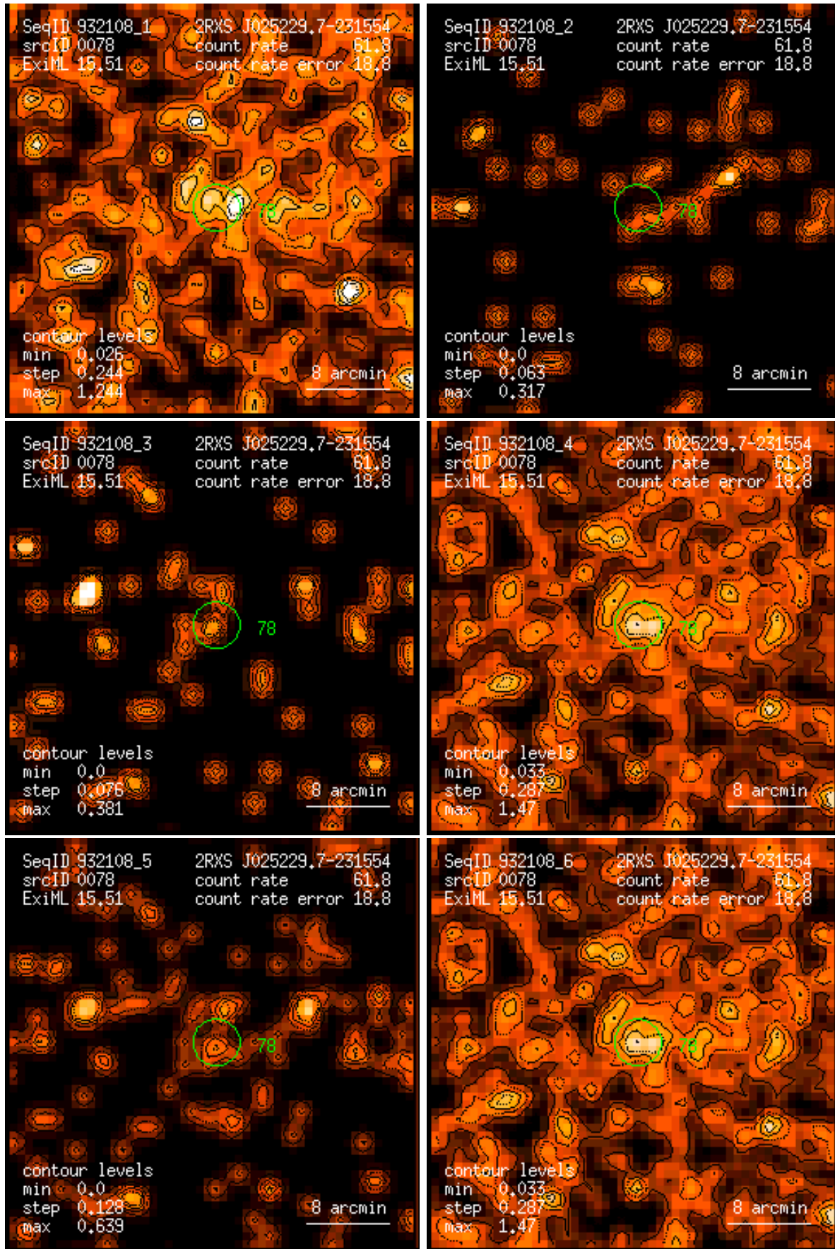
Figure 78: RASS 932108: detection 0078: band rate images, Gaussian filter: (1) PSPC channels 11 – 41, (2) 52 – 90, (3) 91 – 201, (4) 11 – 235, (5) 52 – 201, (6) 11 – 201. Broad band rates in counts/ks. Band rate contour levels in counts/ks/arcmin 2 .
