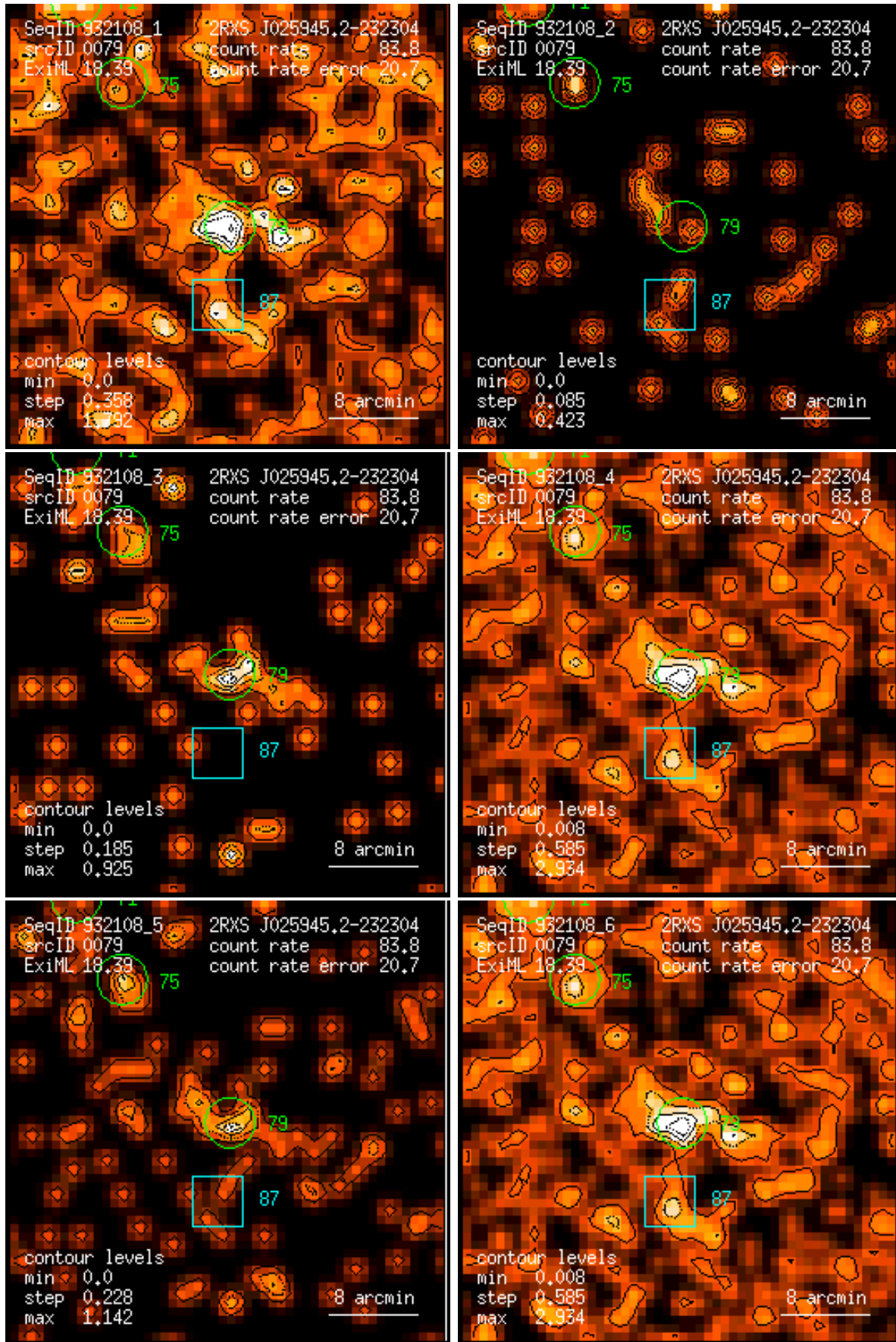
Figure 79: RASS 932108: detection 0079: band rate images, Gaussian filter: (1) PSPC channels 11 – 41, (2) 52 – 90, (3) 91 – 201, (4) 11 – 235, (5) 52 – 201, (6) 11 – 201. Broad band rates in counts/ks. Band rate contour levels in counts/ks/arcmin 2 .
