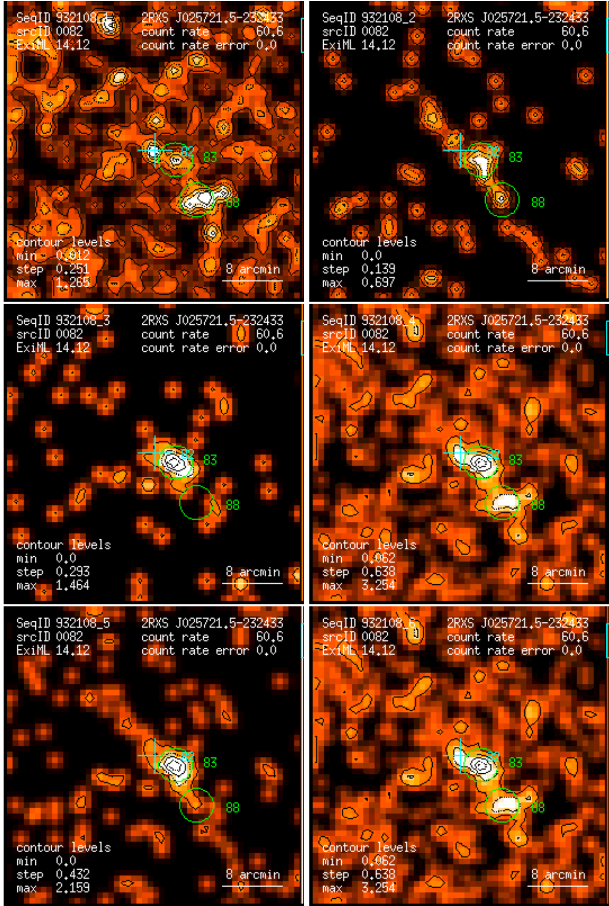
Figure 82: RASS 932108: detection 0082: band rate images, Gaussian filter: (1) PSPC channels 11 – 41, (2) 52 – 90, (3) 91 – 201, (4) 11 – 235, (5) 52 – 201, (6) 11 – 201. Broad band rates in counts/ks. Band rate contour levels in counts/ks/arcmin 2 .
